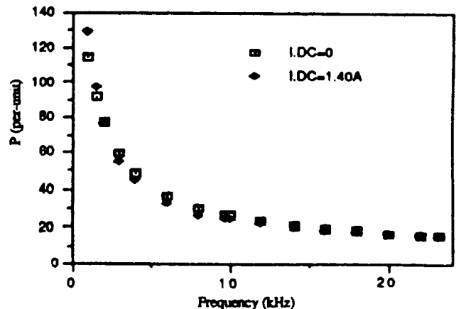
Fig. 9 Power loss vs frequency for closed-slot, cage rotor motor.
