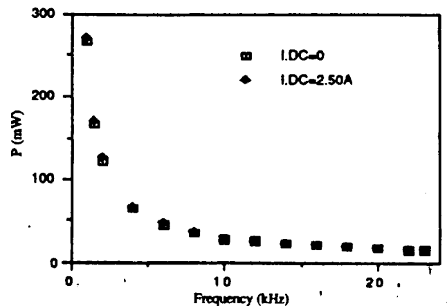
Fig. 8 Power loss vs frequency for open-slot, cage rotor motor.
