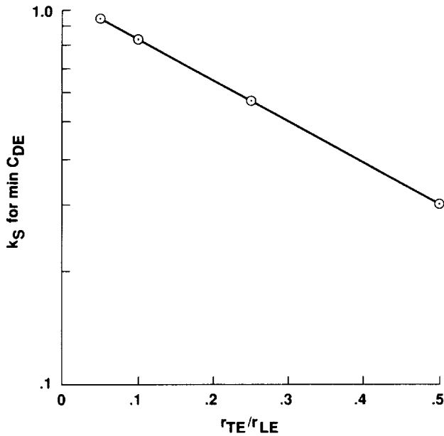
Figure 8. Circulation coefficient for minimum drag vs. rTE/rLE ; \alpha = 0.1 , U_c = 0.164 .
