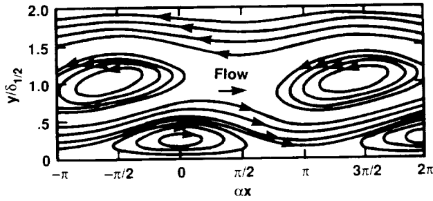
Figure 12. Disturbance streamlines for an ideal wall jet; R = 200 , c = 2 (ref. 36).
