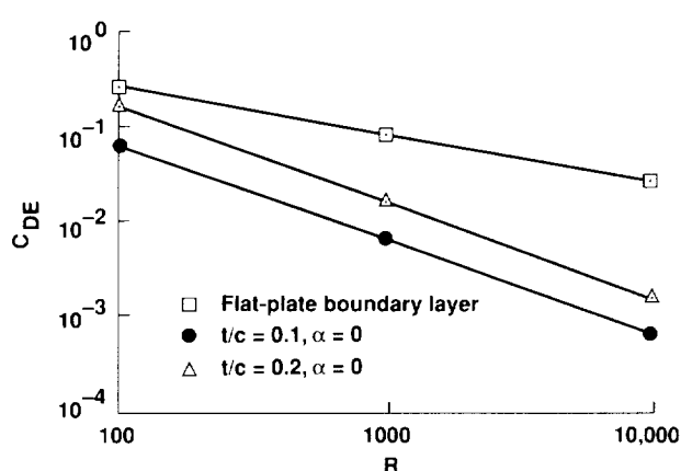
Figure 3. Zero-incidence effective-drag coefficient vs. Reynolds number for a flat-plate boundary layer (two sides) and for symmetrical airfoils (boundary-layer drag excluded on airfoils).
