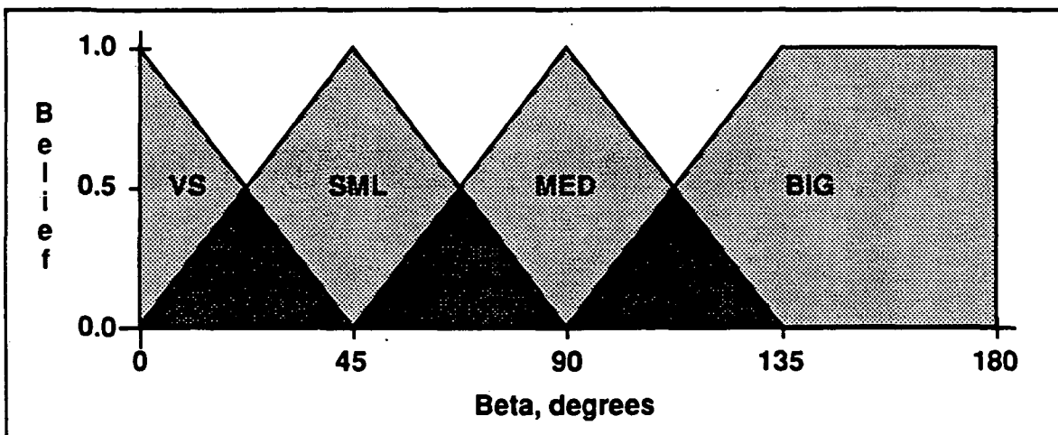
Figure 5.4 - Beta membership functions.
