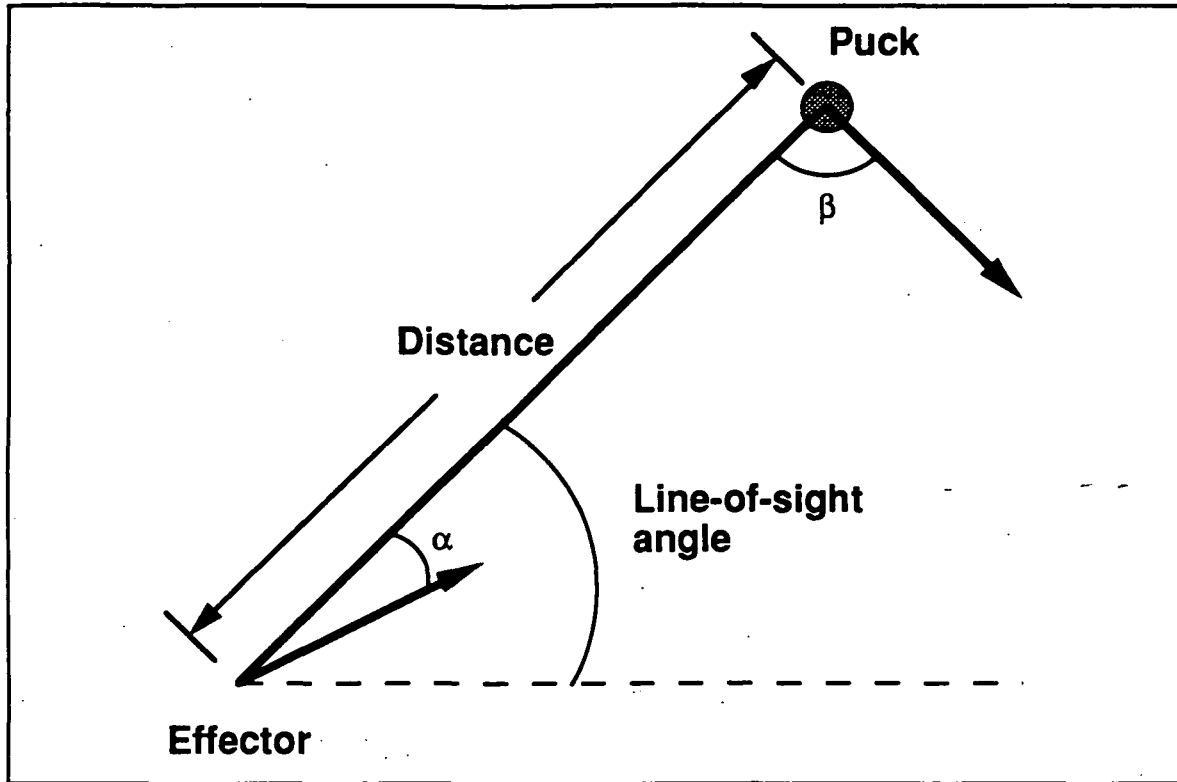
Figure 5.1 - Variable definitions for the fuzzy expert system.
