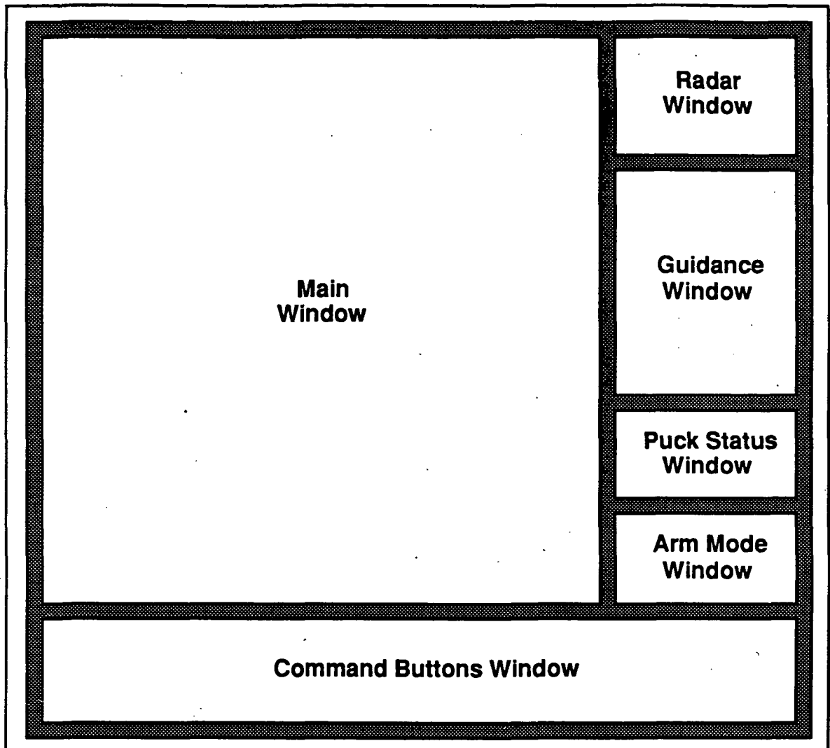
Figure 3.1 - The six windows on the simulation screen.
