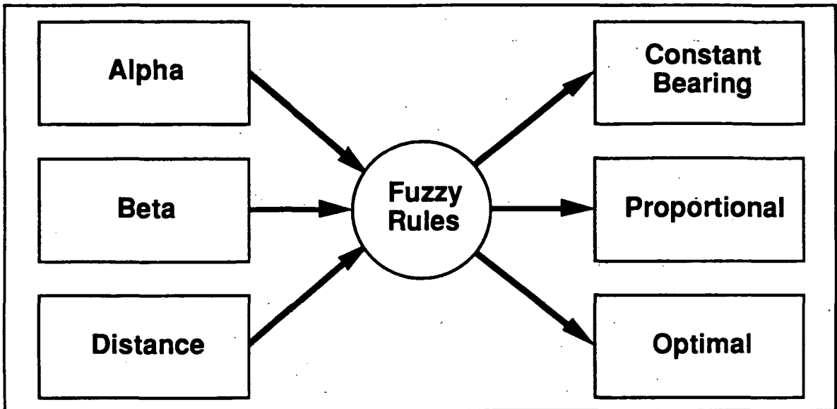
Figure 5.2 - High-level description of the fuzzy expert system.
