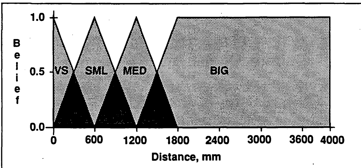
Figure 5.5 - Distance membership functions.
