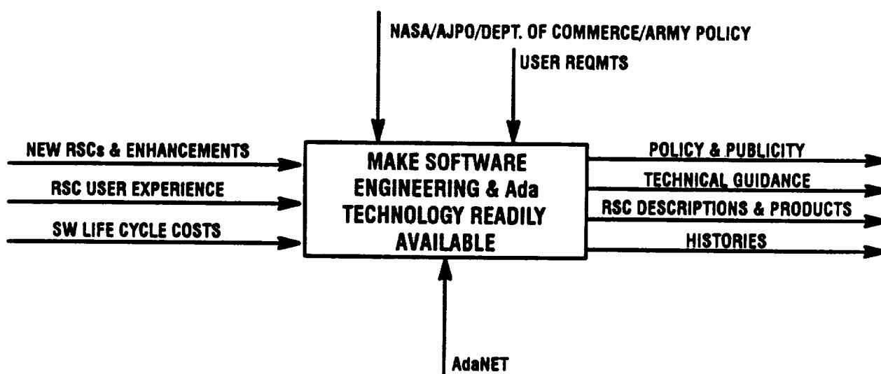
Figure 2. AdaNet Objective
