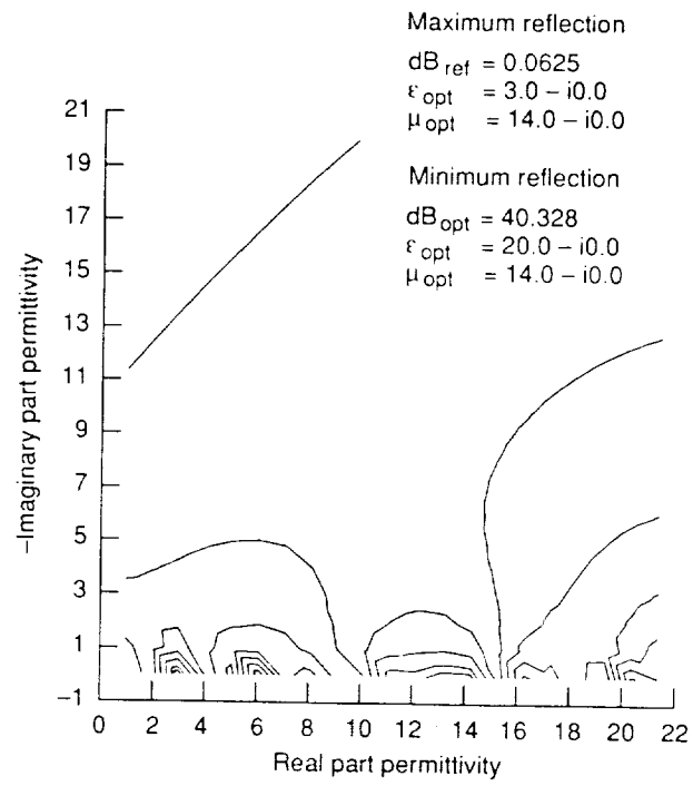
Figure 6.—Acoustic reflection contours for straight duct - final iteration.
