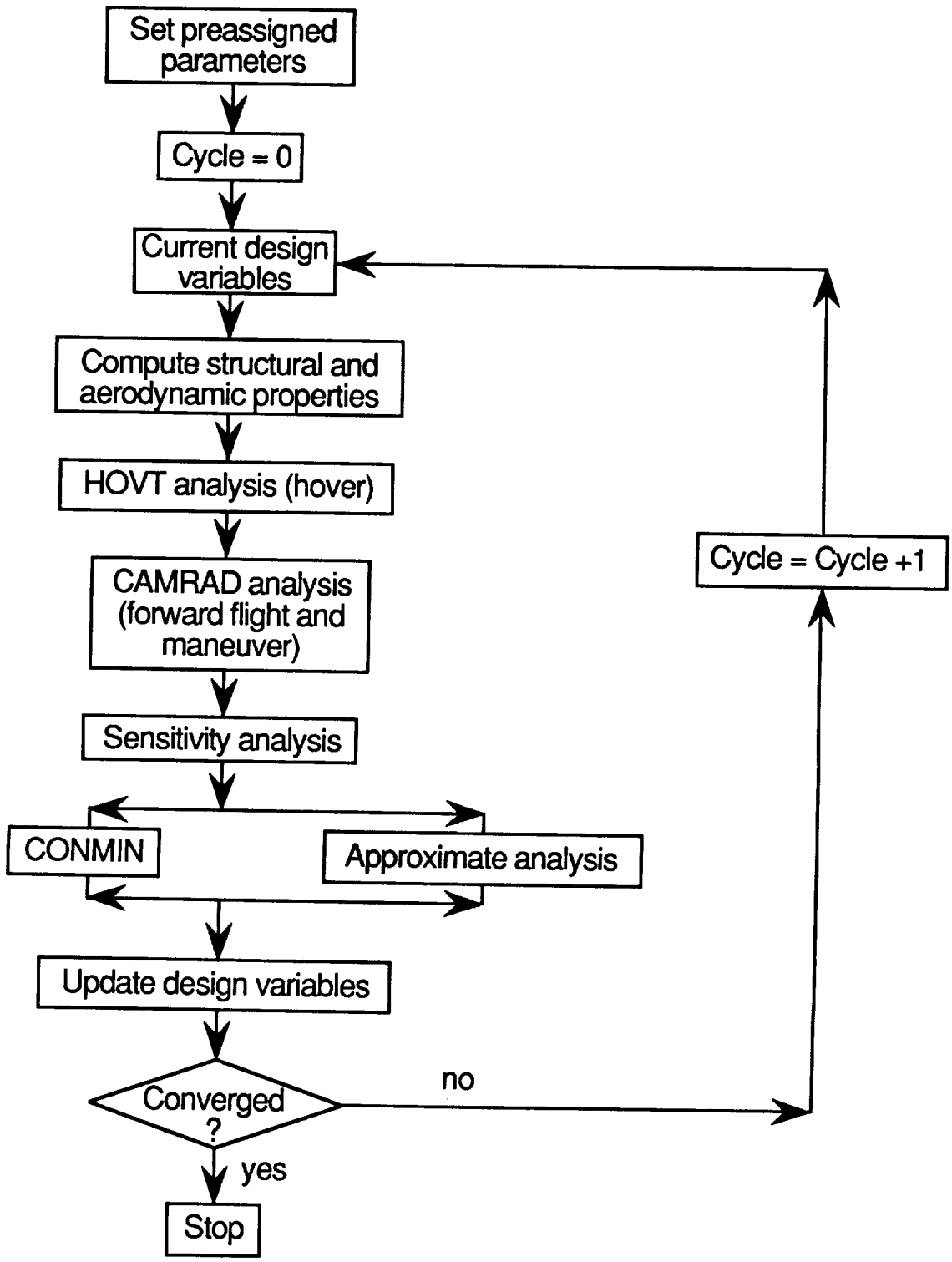
Figure 3. Optimization procedure flow chart.
