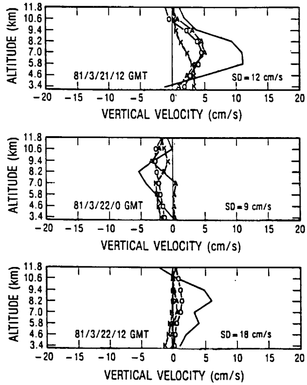
Figure 8. Profiles of the vertical velocity over Platteville, Colorado, from the ST radar (solid line) and the adiabatic (A), kinematic (K), and omega equation (O) methods.
