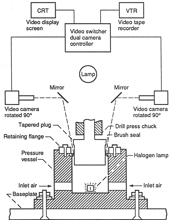
Figure 5.—Test setup.
