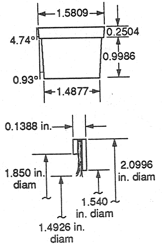
Figure 4.—Tapered plug.
