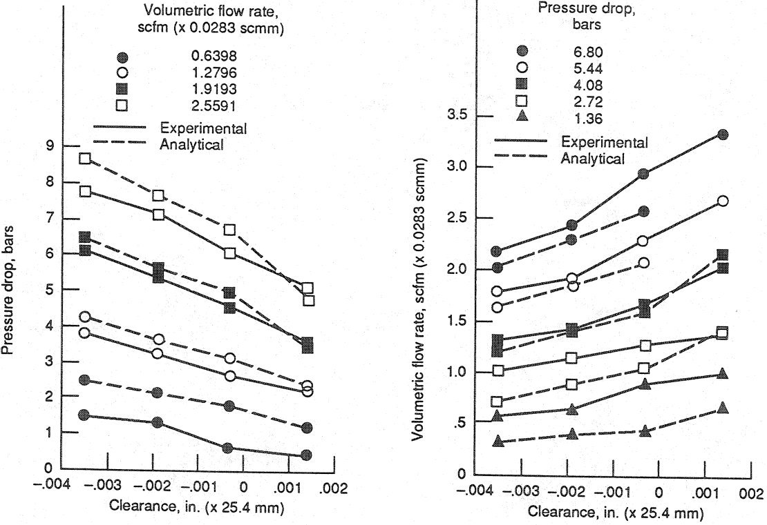
(b) 38-mm (1.5-in.) diameter brush seal.
