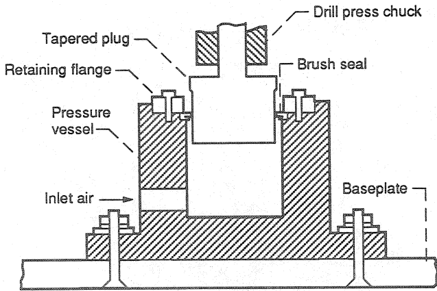
Figure 2.—Test apparatus.
