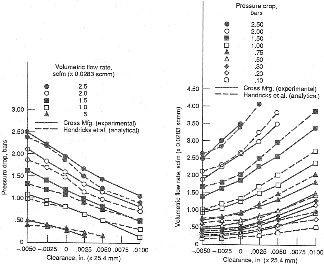
(a) 130-mm (5.1-in.) diameter brush seal.
