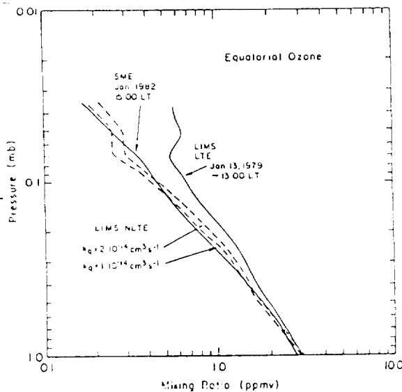
Figure 5. Nimbus 7 LIMS measurements of dayside equatorial ozone (Jan. 13, 1979) before (LIMS LTE) and after (LIMS NLTE) correction for non-LTE effects. The two LIMS NLTE curves are for different quenching rates. Also shown is a comparison between SME dayside ozone measurements in January 1982 and the LIMS measurements corrected for non-LTE effects from (/16/).
