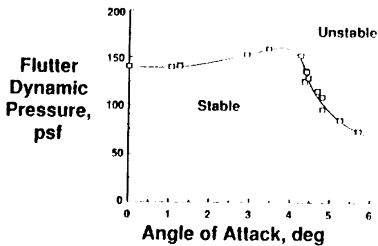
Figure 7. Angle-of-attack effects (M=0.78).
