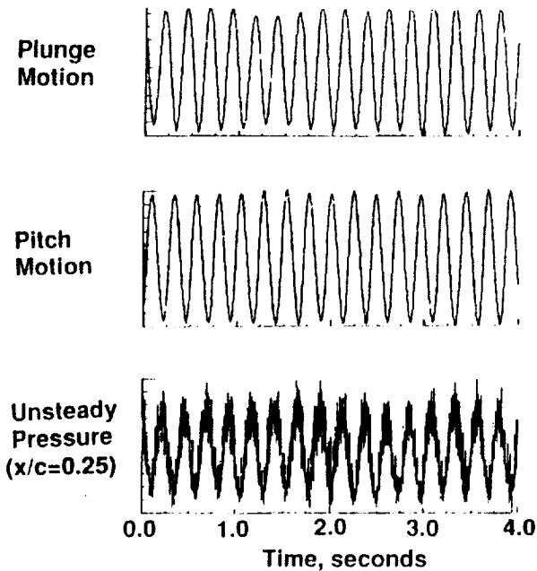
Figure 11. Sample time histories ( M=0.78 , f=4.15 Hz).
