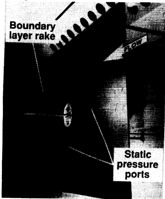
Figure 5. PAPA splitter plate.
