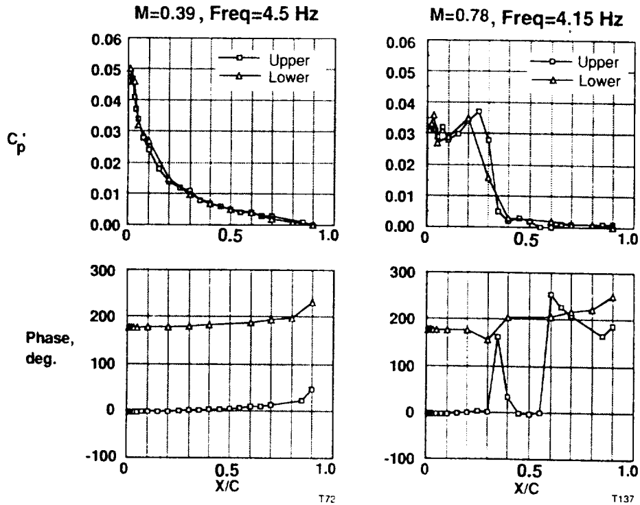
Figure 13. Unsteady pressure response.
