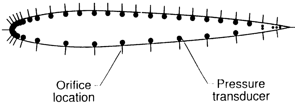
Figure 2. Orifice and pressure transducer locations.
