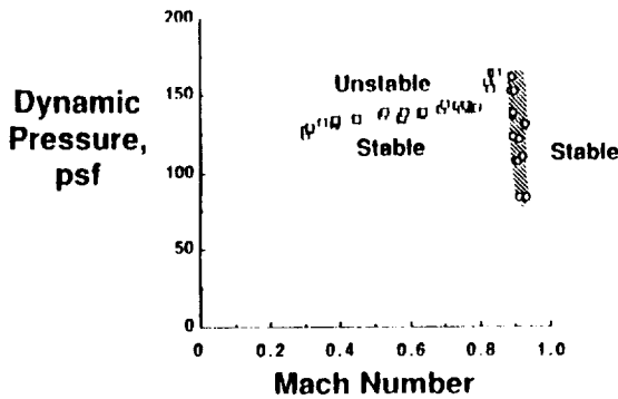
Figure 8. Transonic plunge instability region (alpha=0.0 deg).
