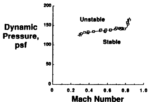
Figure 6. Conventional flutter boundary (alpha=0.0 deg).
