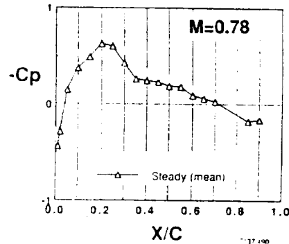
Figure 10. Upper surface steady pressure distribution at 60 percent span.
