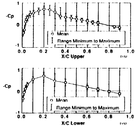
Figure 12. Unsteady pressure statistics ( M=0.78 ).
