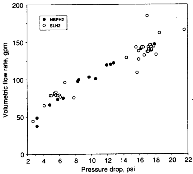
Figure 5.—Volumetric flow rate versus pressure drop for slush hydrogen and normal boiling point hydrogen.
