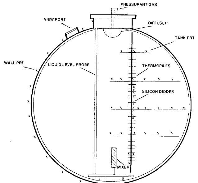
Figure 4.—K-Site slush hydrogen test tank.
