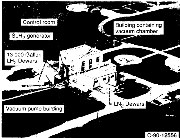
Figure 1.—NASA Plum Brook K-Site facility.
