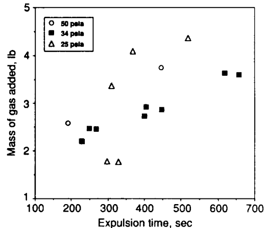
Figure 10.—Pressurant requirements during SLH 2 expulsion; hydrogen pressurant, T gas = 520 R.
