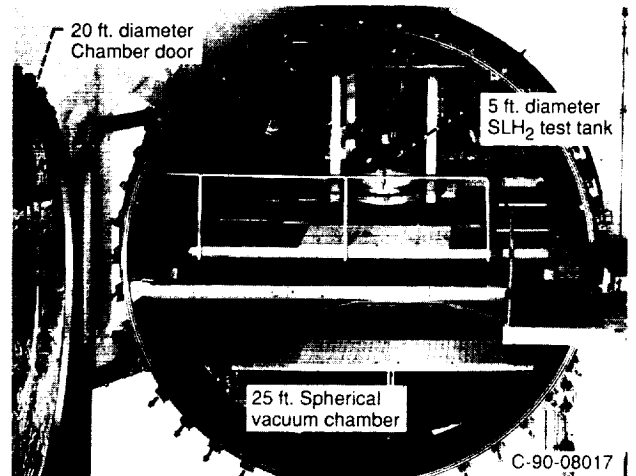
Figure 2.—K-Site 25 foot diameter spherical vacuum chamber.
