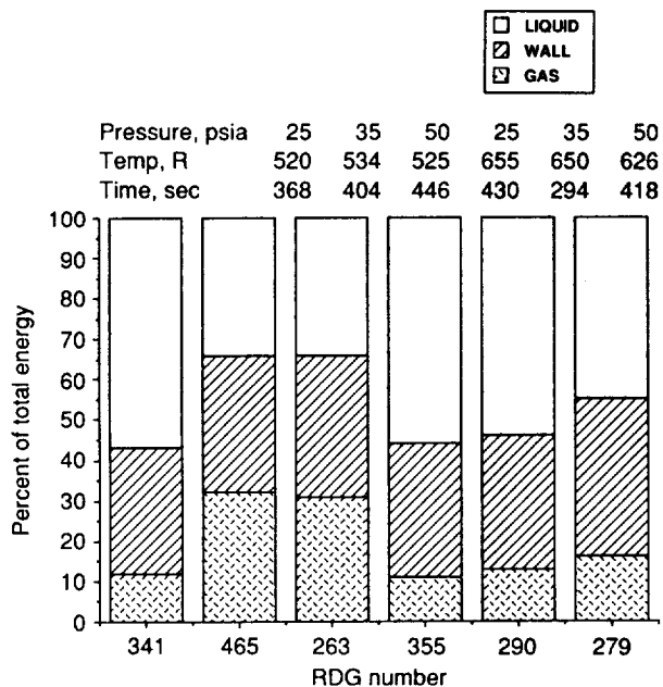
Figure 11.—Slush hydrogen energy balance.
