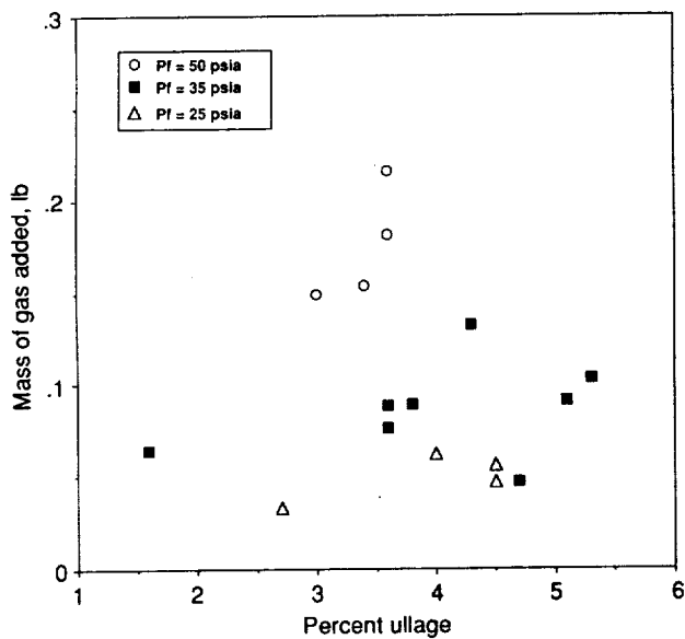
Figure 7.—Pressurant requirements versus ullage fraction: SLH 2 ; hydrogen pressurant, T gas = 520 R.
