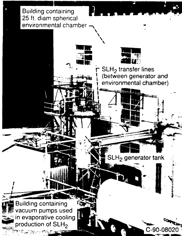
Figure 3.—K-Site SLH 2 production subsystem.
