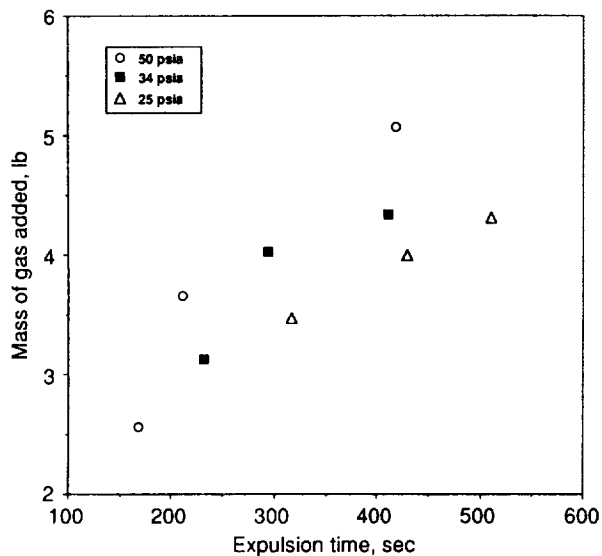
Figure 9.—Pressurant requirements during SLH 2 expulsion. Hydrogen pressurant, T gas = 620.
