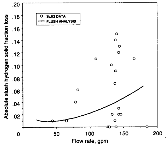
Figure 6.—Comparison of experimental solid fraction loss with FLUSH analysis.
