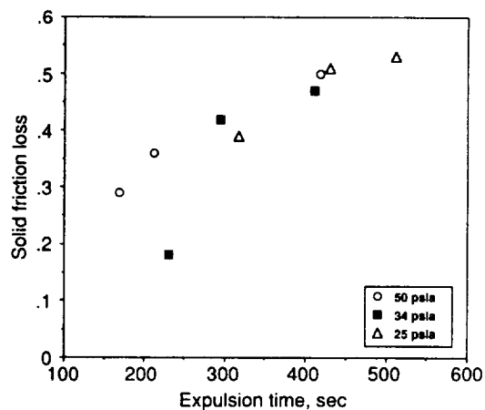
Figure 12.—Slush hydrogen solid fraction loss versus expulsion time; hydrogen pressurant gas, T gas = 620 R. Solid loss based on transfer data solid fraction.
