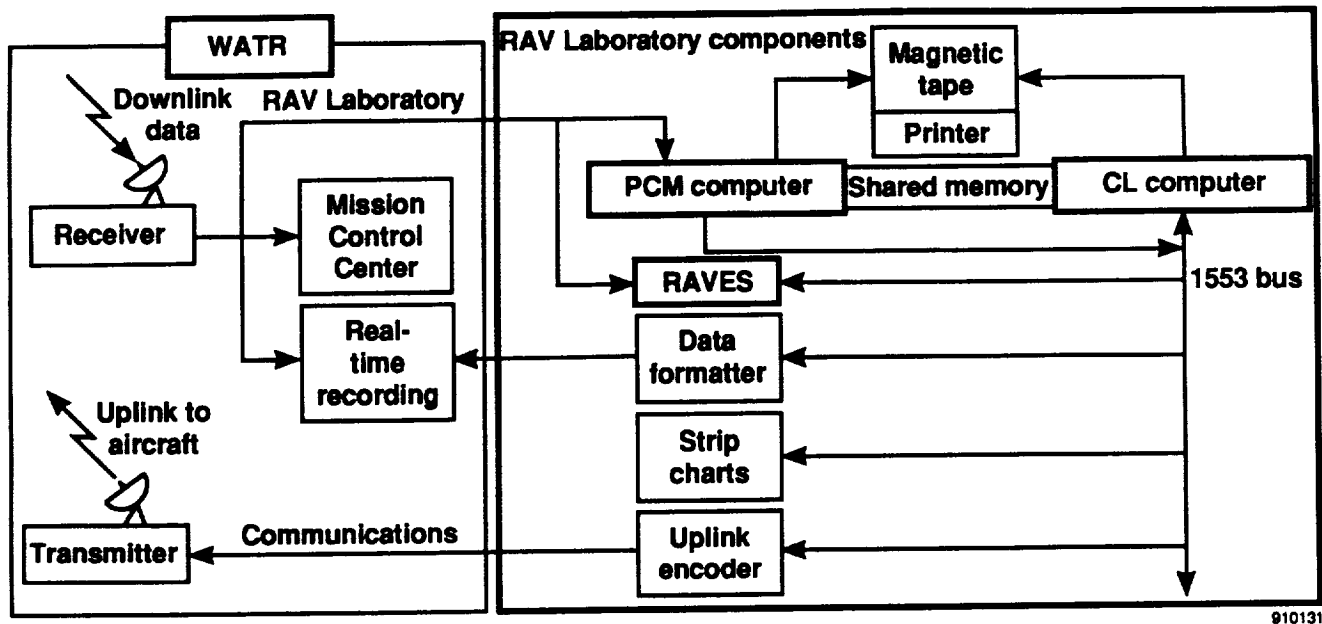
Fig. 3. RAV Laboratory block diagram.
