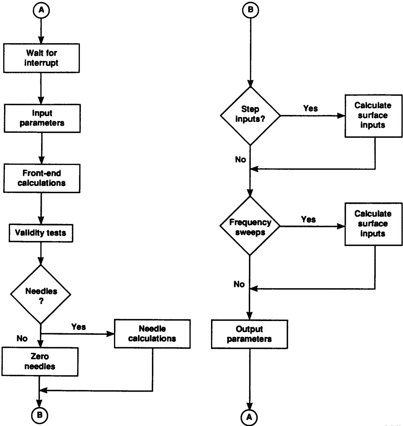
Fig. 5. CL software structure for full RAV application.
