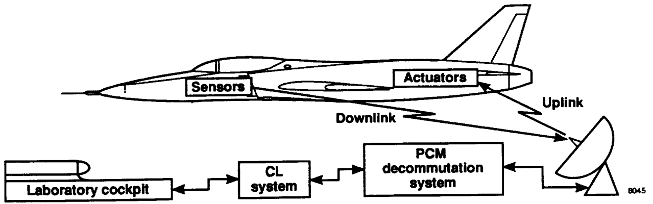
(a) Remotely piloted vehicle.
