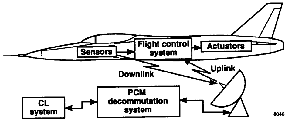
(b) Remotely augmented vehicle.
