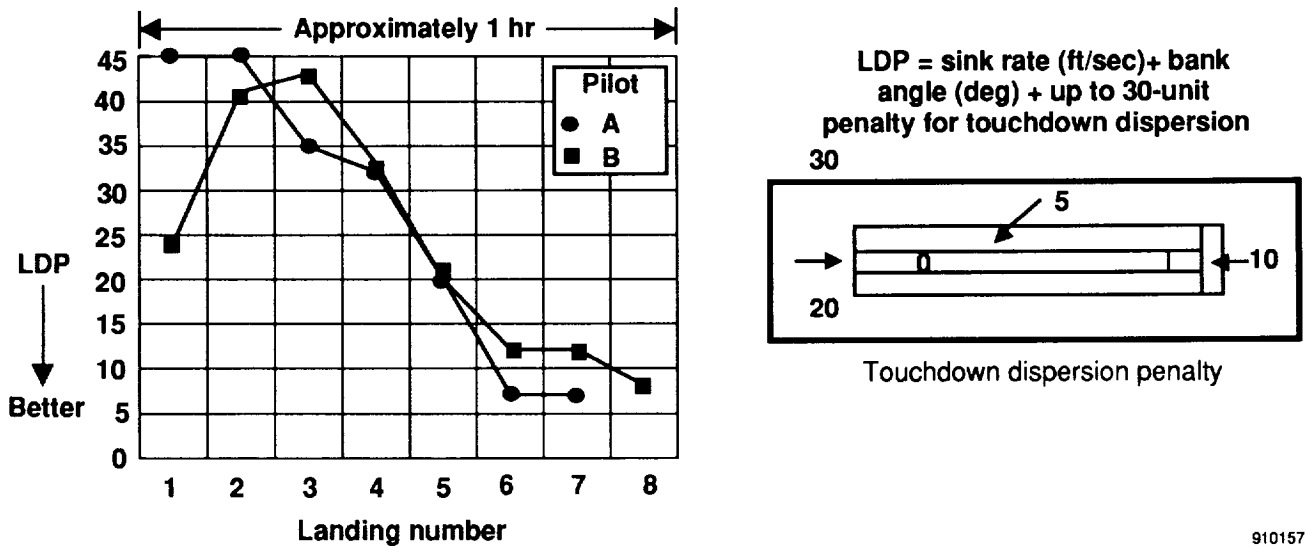
Fig. 10 LDP for F-15 simulation flow with manual throttles-only control, trim airspeed of 170 knots.
