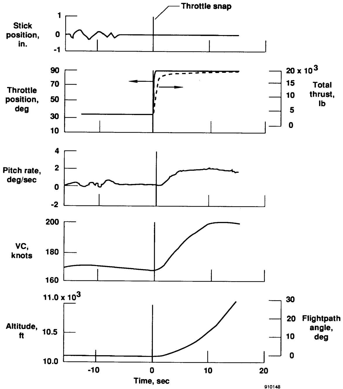
Fig. 2 Flight data time history of response to throttle increase from PLF to intermediate; F-15 airplane, CAS off, control stick free.
