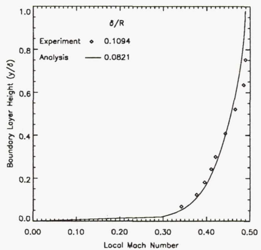
Figure 11. Facility boundary layer profile, M_\infty = 0.5 .
