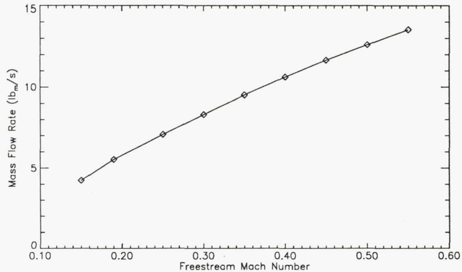
Figure 6. Typical facility operating curve using ambient supply air.
