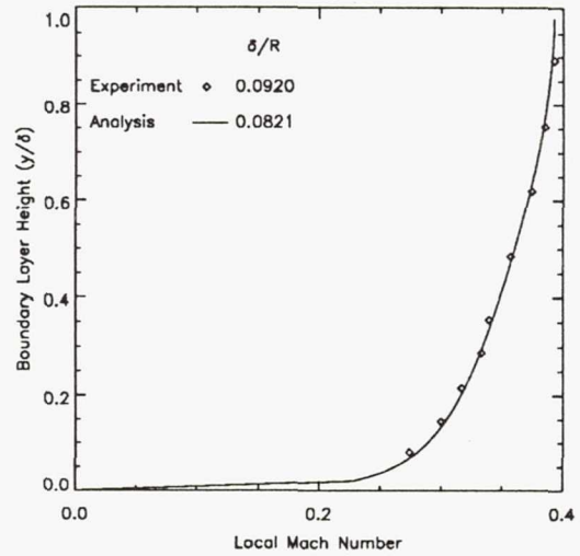
Figure 10. Facility boundary layer profile, M_\infty = 0.4 .
