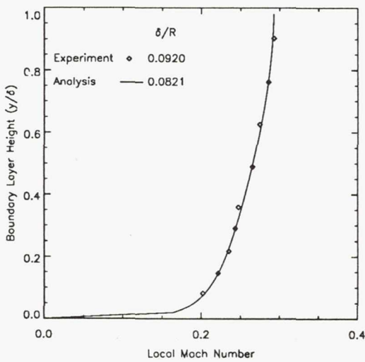
Figure 9. Facility boundary layer profile, M_\infty = 0.3 .
