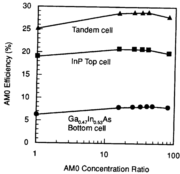
Figure 3. AM0 efficiency versus concentration ratio data for a high-efficiency, three-terminal, concentrator InP/ \text{Ga}_{0.47}\text{In}_{0.53}\text{As} tandem solar cell at 25°C.
