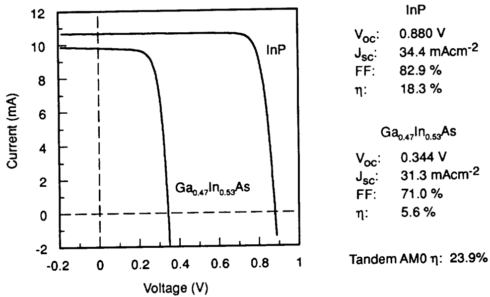
Figure 2. Composite one-sun current-voltage AM0-efficiency data for a high-efficiency, three-terminal, monolithic InP/Ga 0.47 In 0.53 As tandem solar cell at 25°C.
