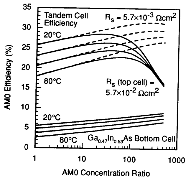
Figure 7. Modeled AMO efficiency as a function of the concentration ratio and temperature for a three-terminal InP/ Ga 0.47 In 0.53 As concentrator tandem cell based on measured subcell parameters. The dashed set of curves illustrate the effect of reducing the InP top cell series resistance by a factor of 10.
