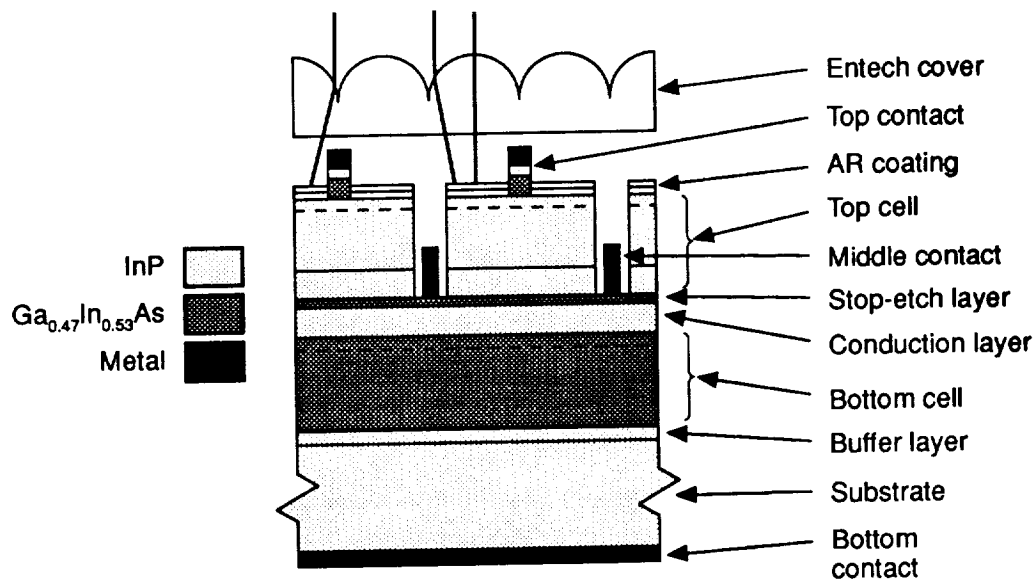
Figure 1. Schematic diagram of the three-terminal, monolithic InP/Ga 0.47 In 0.53 As tandem solar cell structure.
