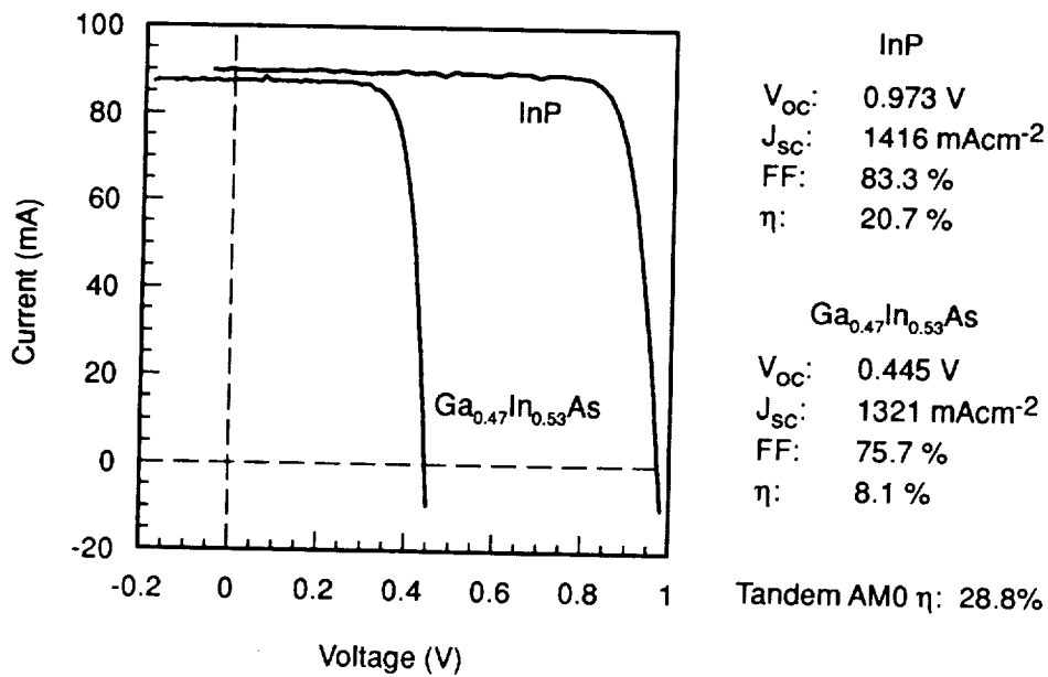
Figure 4. Composite current-voltage data for a three-terminal InP/ \text{Ga}_{0.47}\text{In}_{0.53}\text{As} tandem solar cell at peak AM0 efficiency under 40.3 suns concentration at 25°C.
