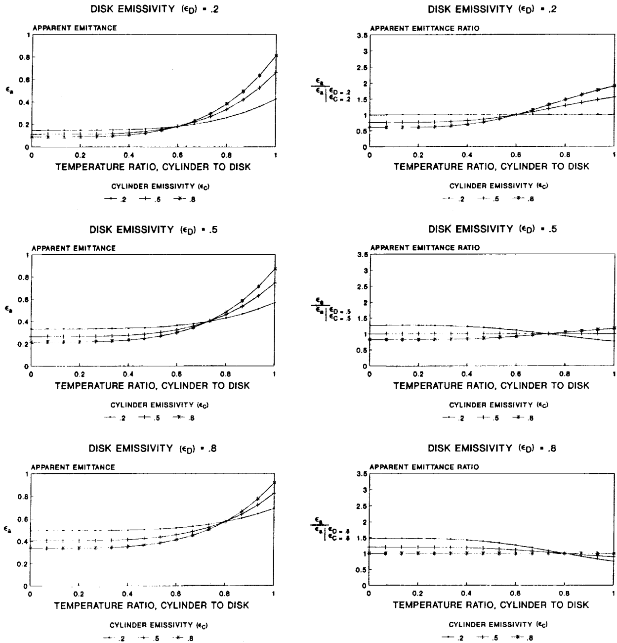
Figure 3.—Apparent emissivity results, L/R = 1.0.
