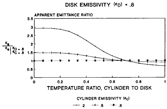
Figure 5.— Apparent emissivity results, L/R = 4.0 .
