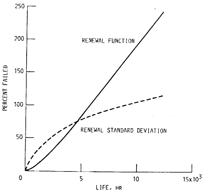
Fig. 4. Renewal function and renewal function standard deviation for a two-parameter Weibull distribution with \theta = 5000 hr, and B = 1.5 .
