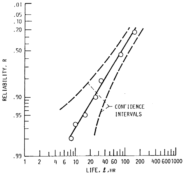
Fig. 2. Two-parameter Weibull probability plot.
