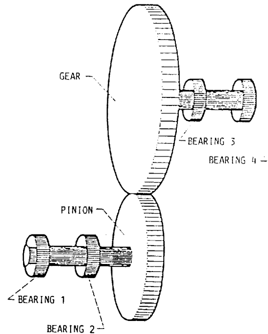
Fig. 1. Single-mesh transmission.
