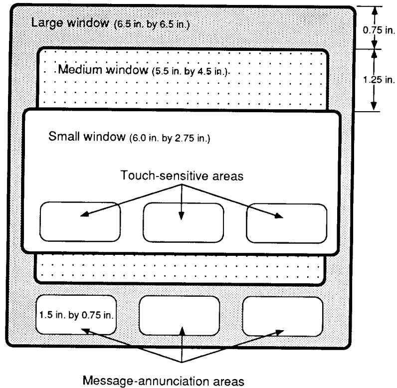
Figure 5. Window format sizes of data link display.
