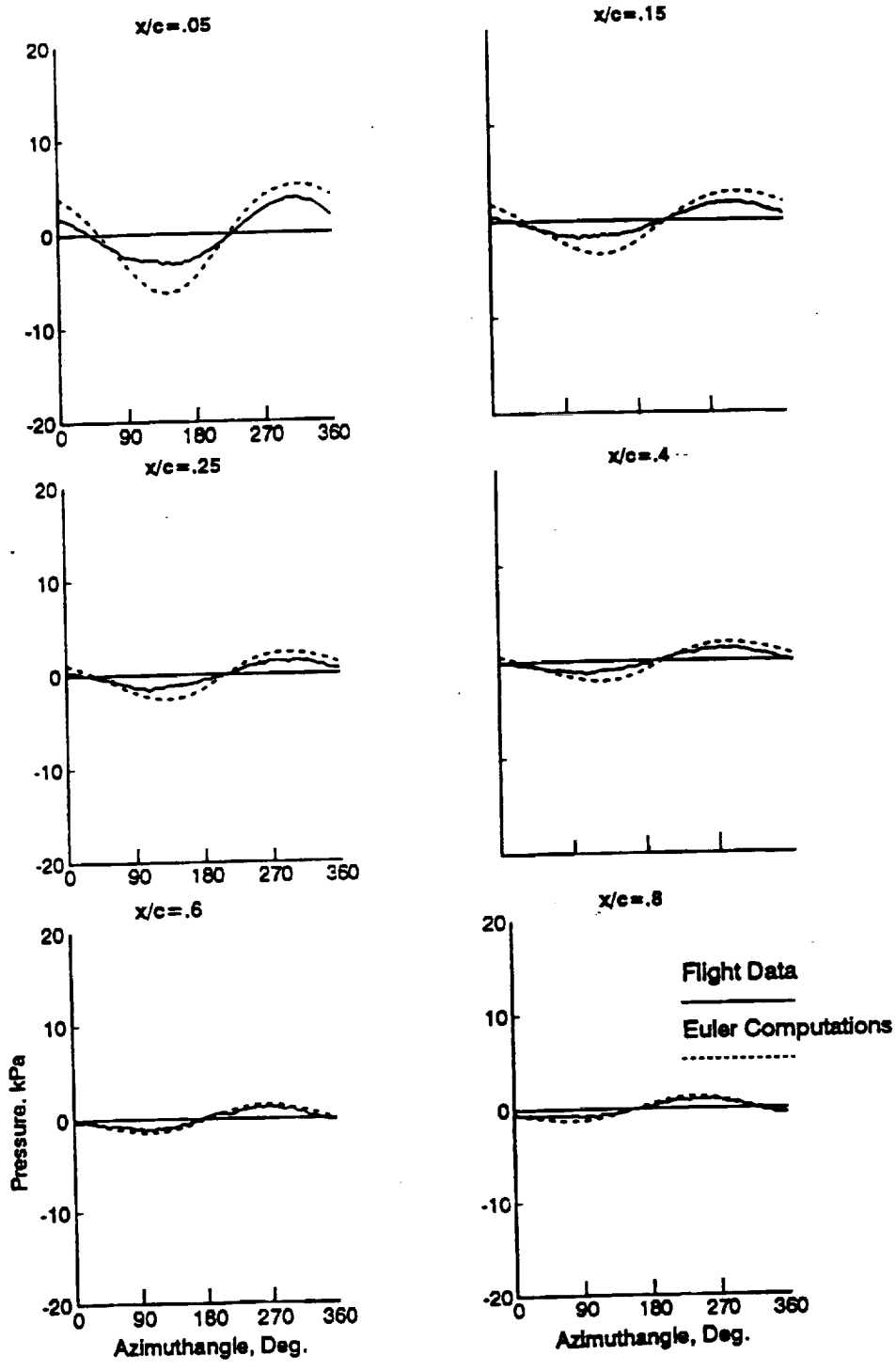
Figure 6. - Predicted and measured presure waveforms at r/R=0.68 on the suction surface. M=0.31 , J=1.6 , \alpha = 8.3^\circ .
