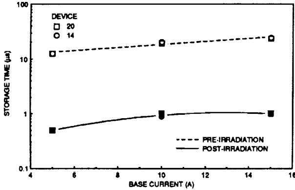
FIGURE 9. COLLECTOR CURRENT STORAGE TIME FOR I_C = 40 A AND V_{CE} = 45 V VERSUS BASE CURRENT FOR NPN TRANSISTOR D60T455010 (450 V/50 A); NEUTRON FLUX = 7.55 \times 10^8 n/cm^2/s , FLUENCE = 1.65 \times 10^{13} n/cm^2 , GAMMA DOSE = 37 Mrad.
