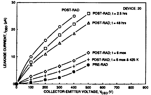
FIGURE 8. COLLECTOR-EMITTER LEAKAGE CURRENT VERSUS COLLECTOR-EMITTER VOLTAGE FOR NPN TRANSISTOR D60T45510 FOR PRE-IRRADIATION, POST-IRRADIATION (FLUENCE = 1.65 \times 10^{13} n/cm^2 , GAMMA DOSE = 37 Mrads), AND THERMAL ANNEALING CONDITIONS. ALL MEASUREMENTS MADE AT 300 K.
