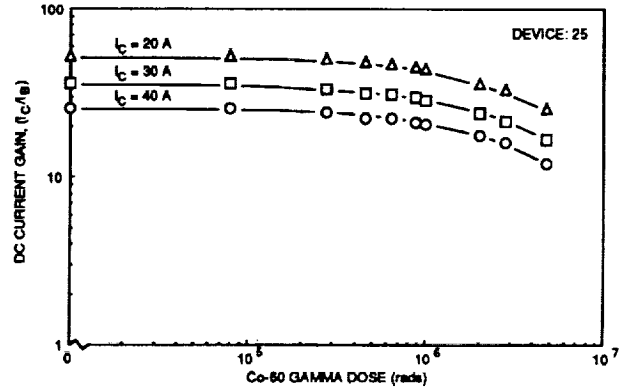
FIGURE 10. DC CURRENT GAIN @ V_{CE} = 2.5 V VERSUS Co-60 GAMMA DOSE FOR NPN TRANSISTOR D60T455010 (450 V/50 A); GAMMA DOSE RATE = 92 Mrads/hr.
