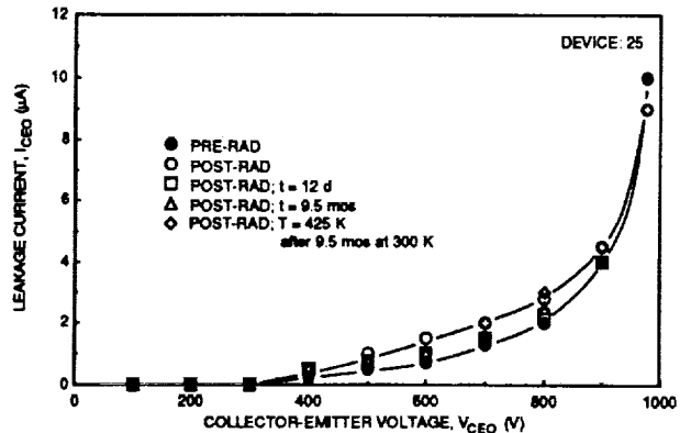
FIGURE 12. COLLECTOR-EMITTER LEAKAGE CURRENT VERSUS COLLECTOR-EMITTER VOLTAGE FOR NPN TRANSISTOR D60T455010 (450 V/50 A) FOR PRE-IRRADIATION, POST-IRRADIATION (GAMMA DOSE = 4.9 Mrads) AND THERMAL ANNEALING CONDITIONS. ALL MEASUREMENTS MADE AT 300 K.
