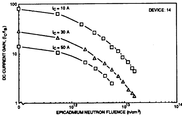
FIGURE 1. DC CURRENT GAIN @ V_{CE} = 2.5 V VERSUS FLUENCE FOR NPN TRANSISTOR D60T455010 (450 V/50 A). FLUX = 7.55 \times 10^8 n/cm 2 s; GAMMA DOSE = 37 krad.
