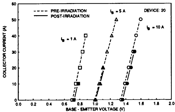
FIGURE 5. BASE-EMITTER VOLTAGE VERSUS COLLECTOR CURRENT FOR NPN TRANSISTOR D60T455010 (450 V/50 A); NEUTRON FLUX = 7.55 \times 10^8 n/cm 2 s, FLUENCE = 1.65 \times 10^{13} n/cm 2 , TOTAL GAMMA DOSE = 37 krad.
