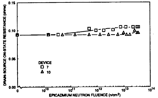
FIGURE 14. DRAIN-SOURCE ON-STATE RESISTANCE FOR I_D = 30 A AND V_{GS} = 10 V VERSUS EPISCADMIUM NEUTRON FLUENCE FOR N-CHANNEL IRF250 (200 V/30 A); NEUTRON FLUX = 3.78 \times 10^7 TO 2.27 \times 10^9 n/cm^2 , GAMMA DOSE = 85 krads.
