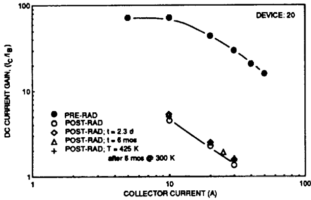
FIGURE 3. DC CURRENT GAIN @ V_{CE} = 2.5 V VERSUS COLLECTOR CURRENT FOR PRE-IRRADIATION, POST-IRRADIATION (FLUX = 7.55 \times 10^8 n/cm 2 s, FLUENCE = 1.65 \times 10^{13} n/cm 2 , GAMMA DOSE = 37 krad), AND THERMAL ANNEALING CONDITIONS FOR NPN TRANSISTOR D60T455010. ALL MEASUREMENTS MADE AT 300 K.
