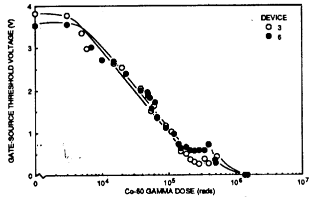
FIGURE 16. GATE-SOURCE THRESHOLD VOLTAGE VERSUS GAMMA DOSE FOR N-CHANNEL IRF250 (200 V/30 A); GAMMA DOSE RATE = 33.8 TO 62.1 krads/hr.
