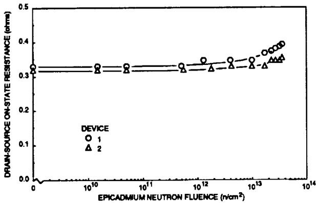
FIGURE 13. DRAIN-SOURCE ON-STATE RESISTANCE FOR I_D = 15 A AND V_{GS} = 10 V VERSUS EPISCADMIUM NEUTRON FLUENCE FOR N-CHANNEL MTM15N50 (500 V/15 A); NEUTRON FLUX = 3.78 \times 10^7 TO 2.27 \times 10^9 n/cm^2 , GAMMA DOSE = 85 krads.
