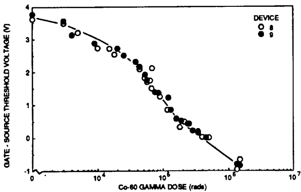
FIGURE 15. GATE-SOURCE THRESHOLD VOLTAGE VERSUS GAMMA DOSE FOR N-CHANNEL MTM15N50 (500 V/15 A); GAMMA DOSE RATE = 33.8 TO 62.1 krads/hr.
