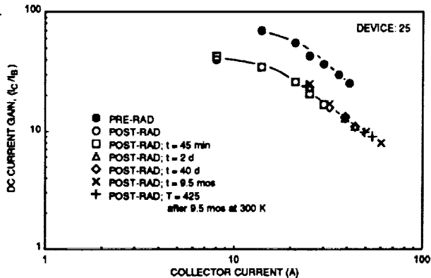
FIGURE 11. DC CURRENT GAIN @ V_{CE} = 2.5 V VERSUS COLLECTOR CURRENT FOR NPN TRANSISTOR D60T455010 (450 V/50 A) FOR PRE-IRRADIATION, POST-IRRADIATION (GAMMA DOSE = 4.9 Mrads) AND THERMAL ANNEALING CONDITIONS. ALL MEASUREMENTS MADE AT 300 K.
