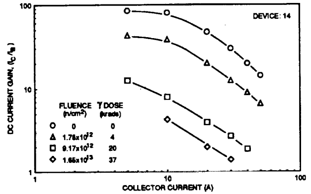
FIGURE 2. DC CURRENT GAIN @ V_{CE} = 2.5 V VERSUS COLLECTOR CURRENT FOR VARIOUS EPISCADMIUM NEUTRON FLUENCES AND BACKGROUND GAMMA DOSES FOR NPN TRANSISTOR D60T455010 (450 V/50 A); NEUTRON FLUX = 7.55 \times 10^8 n/cm 2 s.
