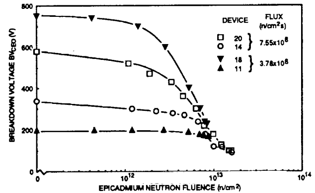
FIGURE 6. BREAKDOWN VOLTAGE BV_{CEO} @ I_{CEO} = 10 \mu A VERSUS FLUENCE FOR NPN TRANSISTOR D60T455010 (450 V/50 A), GAMMA DOSE: (20 & 14) = 37 krad; (18 & 11) = 18.5 krad.
