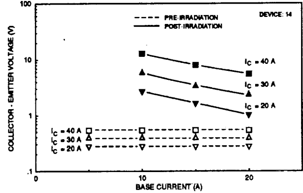
FIGURE 4. COLLECTOR - EMITTER VOLTAGE VERSUS BASE CURRENT FOR NPN TRANSISTOR D60T455010 (450 V/50 A); NEUTRON FLUX = 7.55 \times 10^8 n/cm 2 s, FLUENCE = 1.65 \times 10^{13} n/cm 2 ; TOTAL GAMMA DOSE = 37 krad.
