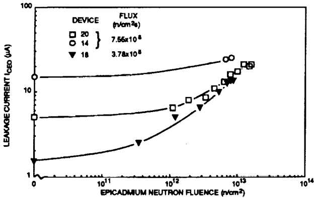
FIGURE 7. LEAKAGE CURRENT I_{CEO} @ V_{CE0} = 400 VDC VERSUS FLUENCE FOR NPN TRANSISTOR D60T45510 (450 V/50 A); TOTAL GAMMA DOSE (20 & 14) = 37 Mrads; (18) = 18.5 Mrads.
