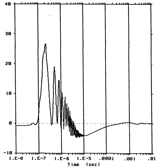
Fig.16 CFC Aircraft Typical CW Predicted Wiring Transient (Component H)
