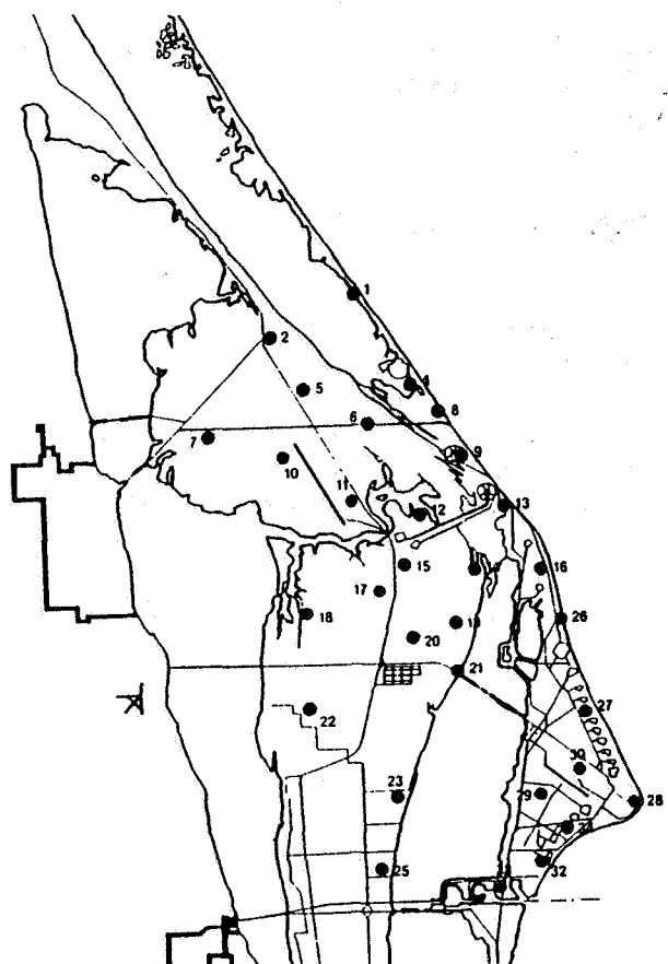
Fig. 4. Ground Based Field Mill (GBFM) Locations at CCAFS and KSC.
