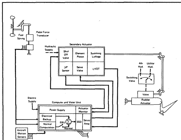
FIGURE 1 Typical FBW System
