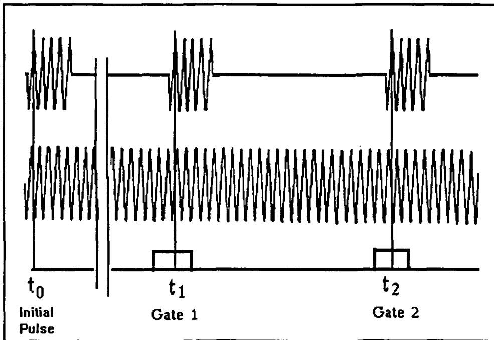
Figure 4. Waveforms used in Matec MBS-8000 System for velocity measurements.
