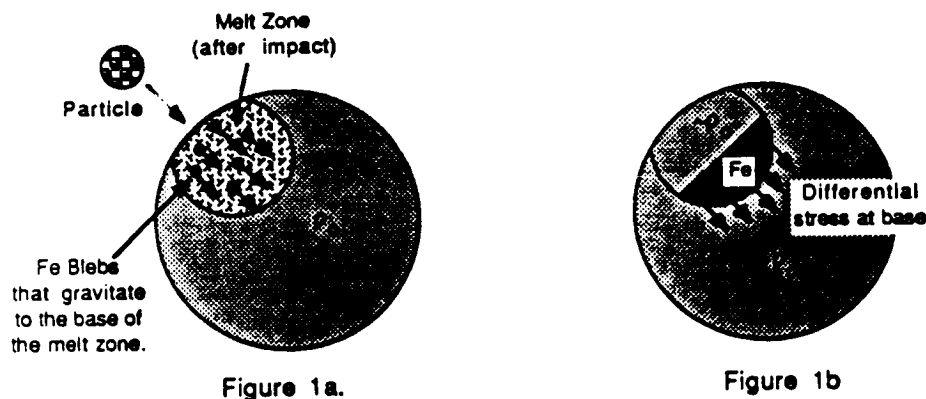
Figure 1. Impact Induced Core Formation
