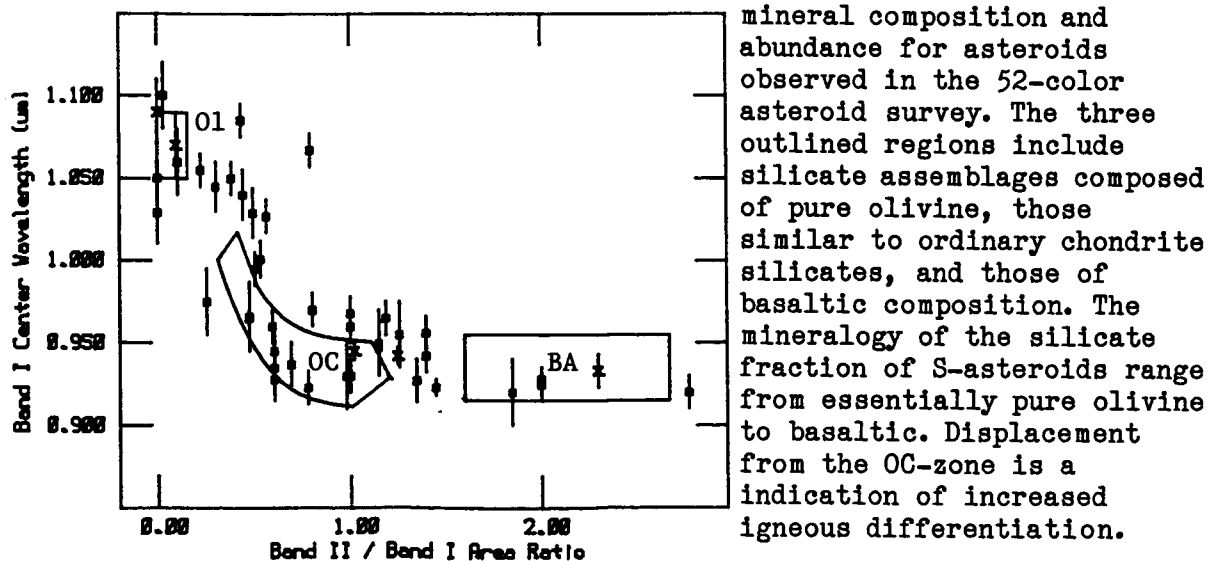
Figure 1: The distribution of two spectral parameters related to silicate mineral composition and abundance for asteroids observed in the 52-color asteroid survey. The three outlined regions include silicate assemblages composed of pure olivine, those similar to ordinary chondrite silicates, and those of basaltic composition. The mineralogy of the silicate fraction of S-asteroids range from essentially pure olivine to basaltic. Displacement from the OC-zone is a indication of increased igneous differentiation.
