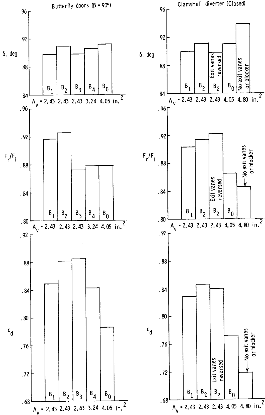
Figure 22. Butterfly door and clamshell diverter ventral nozzle internal performance with various nozzle exit blockers at NPR = 3.0 and nozzle exit vanes at 90°.
