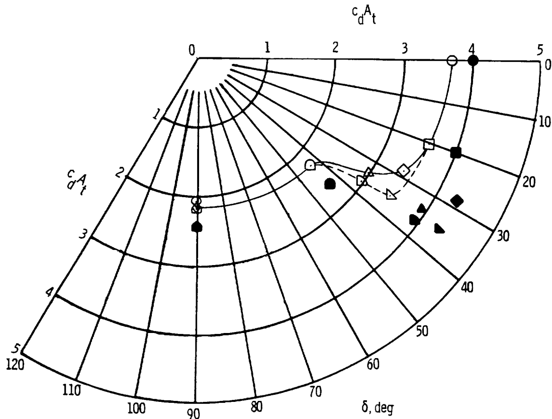
Figure 30. Variation of effective throat area c_d A_t with resultant-thrust-vector angle from cruise to vertical flight for 2D-CD rear nozzle configurations with butterfly door ventral nozzle at NPR = 3.0. Dashed line indicates extrapolation and fairing of data for 30° rear nozzle through transition range.
