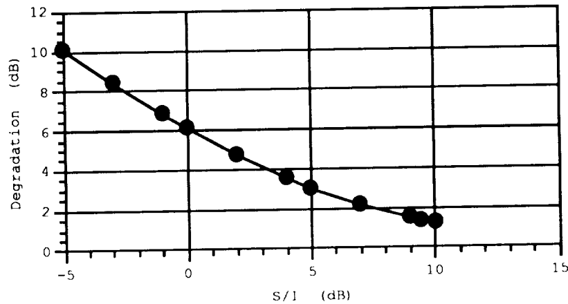
Figure 2. Computed relationship between degradation and S/I for the case where the desired user is the Space Shuttle Orbiter using channel 3, 50 Mbps coded, and the interferer (assumed to be on the TDRS SA antenna boresight) is Space Station Freedom using the 50 Mbps (I+Q) link. The desired user and interferer links are cross polarized with an assumed polarization rejection of the interfering signal of 15 dB on the TDRS SA antenna boresight.
