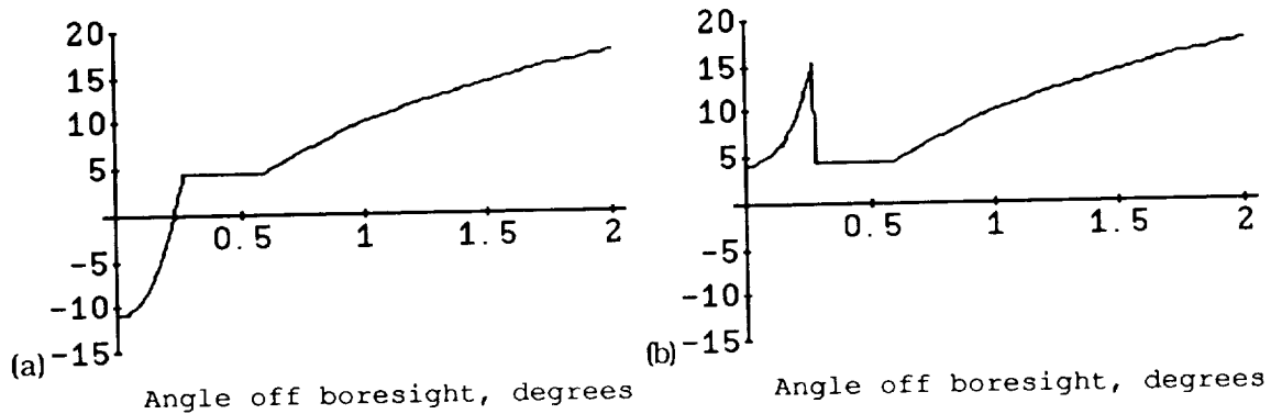
Figure 4. S/I as a function of interferer's angle off boresight: (a) for the case where desired user and interferer have the same polarization, and (b) for a representative case where desired user and interferer are oppositely polarized, showing the effect, on the interfering signal, of TDRS antenna gain and polarization rejection.
