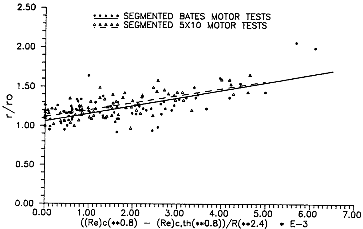
Fig. 9. Burning Rate Augmentation vs. (Re\ No. (**0.8) - Re\ No.,th(**0.8))/R(**2.4)
