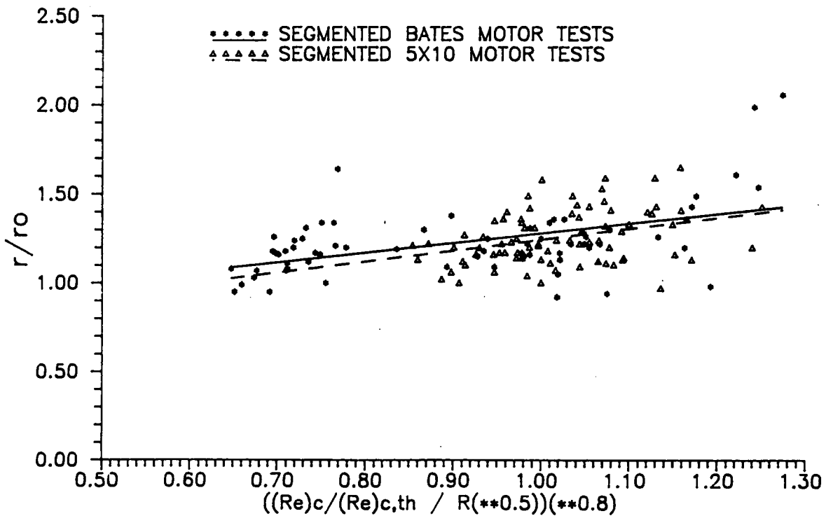
Fig. 10. Burning Rate Augmentation vs. (Re\ No./Re\ No.,th/R(**0.5))(**0.8)
