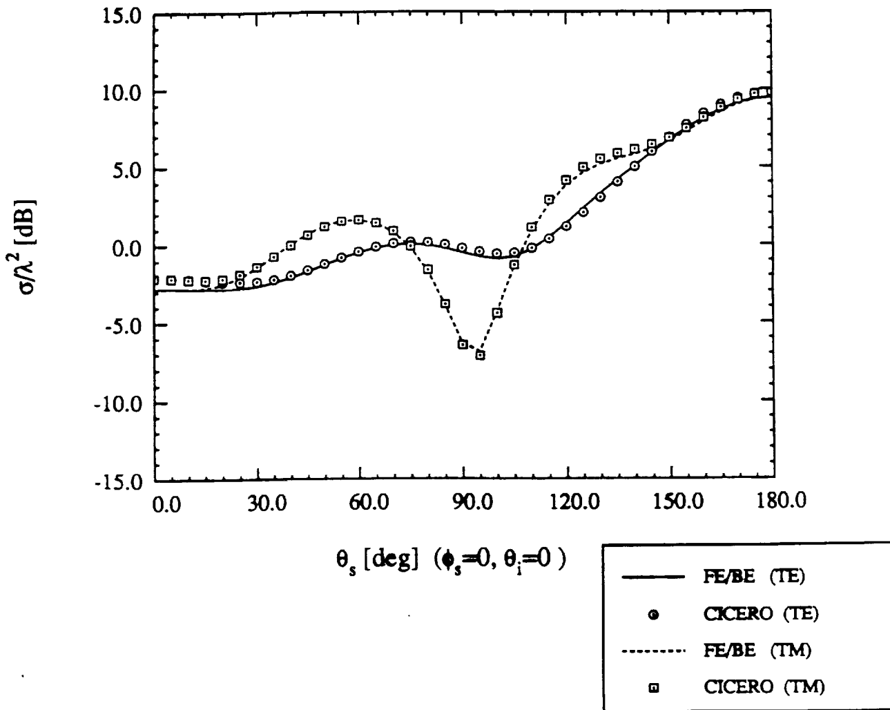
Conducting Sphere ( \rho=0.5\lambda )
