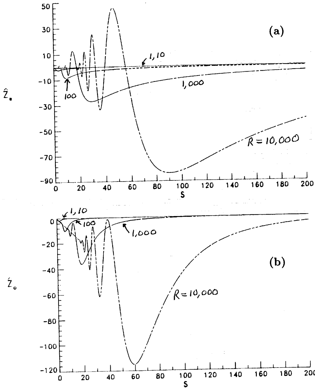
Figure 9. Plot of (a) Z_0 and (b) Z_0 versus s for Sc = 1 and various values of the vortex Reynolds number.
