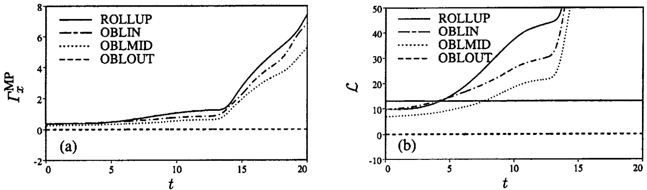
Figure 37. Time development of (a) streamwise circulation ( \Gamma_x^{\text{MP}} ), and (b) the Lin and Corcos collapse parameter \mathcal{L} . The solid line at \mathcal{L} = 13.1 in (b) represents the Lin and Corcos collapse criterion.
