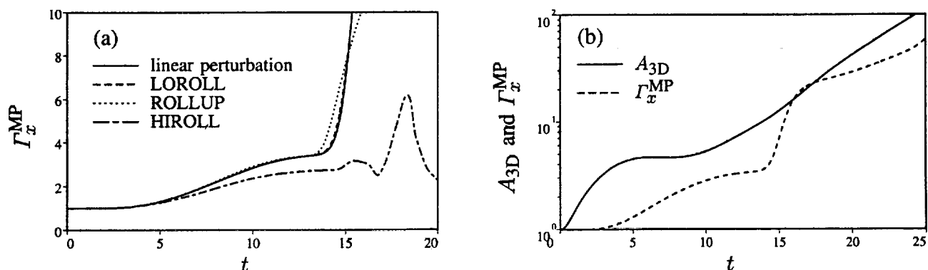
Figure 52. Time development of (a) \Gamma_x^{\text{MP}} of the linear perturbation and nonlinear flows, and (b) A_{3D} and \Gamma_x^{\text{MP}} of the linear perturbation. All quantities are normalized by their values at t = 0 .
