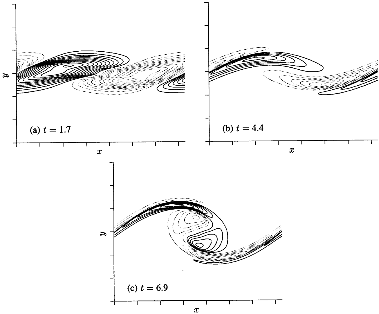
Figure 40. Contour plots of streamwise vorticity in the RP of OBL0UT (it is zero in the BP). Contour increments are (a) \pm 0.03 , (b) \pm 0.2 , and (c) \pm 0.3 . Solid contours indicate positive vorticity, dotted contours indicate negative vorticity, and tic marks are at \delta_\omega^0 intervals.
