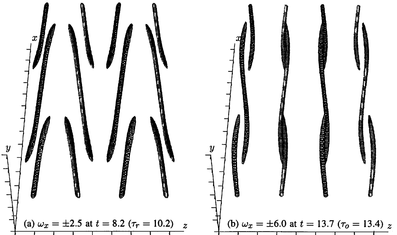
Figure 34. Surfaces of constant streamwise vorticity magnitude in OBLIN. Cross-hatched surfaces represent negative \omega_x , and shaded surfaces represent positive \omega_x . Periodicity has been used to extend the domain in both the streamwise and spanwise directions. Tic marks are at \delta_\omega^0 intervals.
