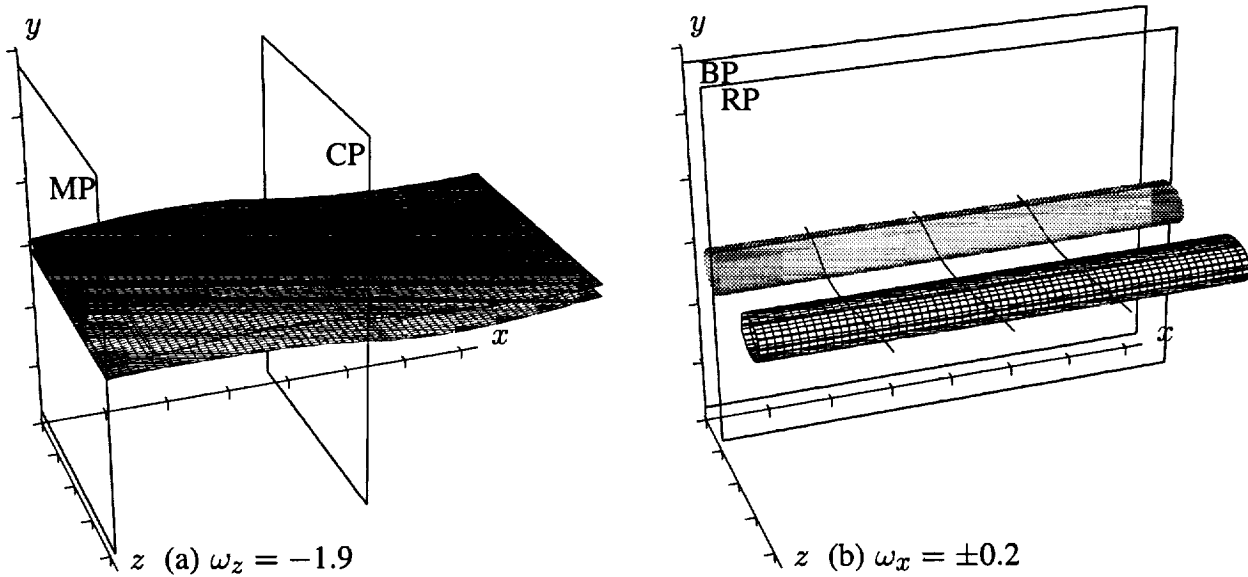
Figure 6. Surfaces of constant vorticity magnitude and vortex lines at t = 0 . Cross-hatched surfaces represent negative vorticity levels, shaded surfaces represent positive vorticity levels, and tic marks are at \delta_\omega^0 intervals. Also shown are the special planes MP, CP, BP, and RP.
