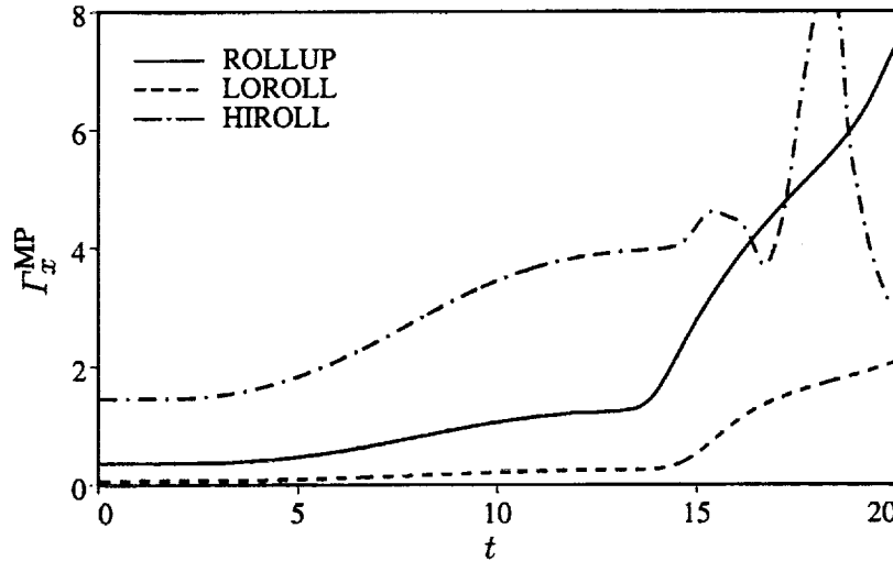
Figure 26. Time development of streamwise circulation in the MP ( \Gamma_x^{MP} ) for ROLLUP, LOROLL, and HIROLL.
