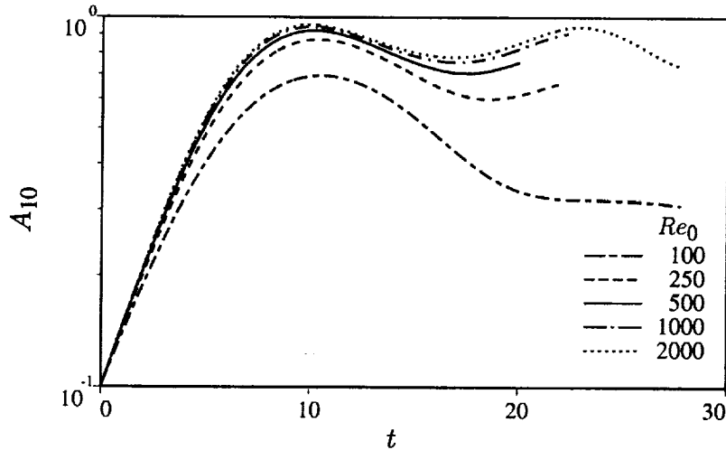
Figure 2. Time development of A_{10} at various Reynolds numbers (viscous eigenfunction disturbance profiles were used).
