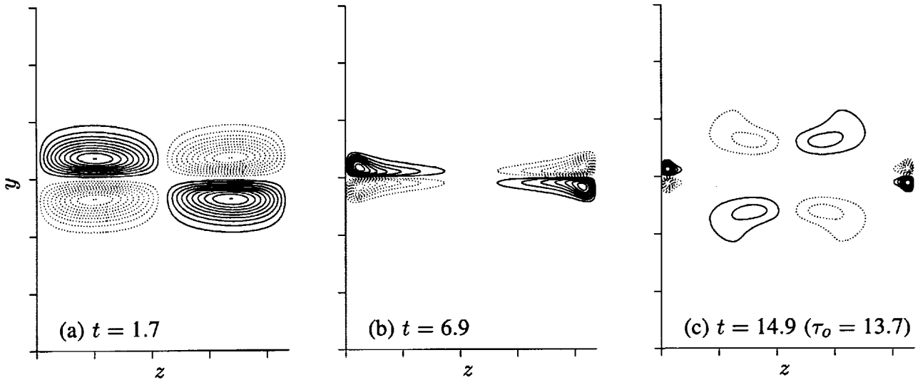
Figure 41. Contour plots of streamwise vorticity in the MP of OBLIOUT. Contour increments are (a) \pm 0.02 ; and (b),(c) \pm 0.3 . Solid contours indicate positive vorticity, dotted contours indicate negative vorticity, and tic marks are at \delta_\omega^0 intervals.
