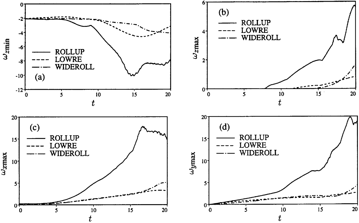
Figure 29. Time development of vorticity component extrema for ROLLUP, LOWRE, and WIDEROLL. Note that \omega_{xmin} and \omega_{ymin} are equal in magnitude but opposite in sign to \omega_{xmax} and \omega_{ymax} .
