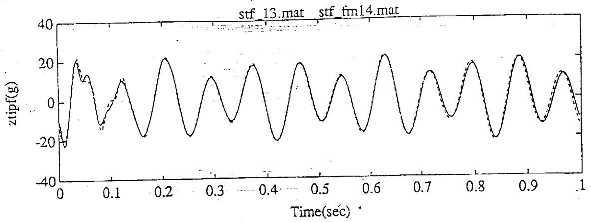
a) Acceleration near forward end of tip missile, g's.
