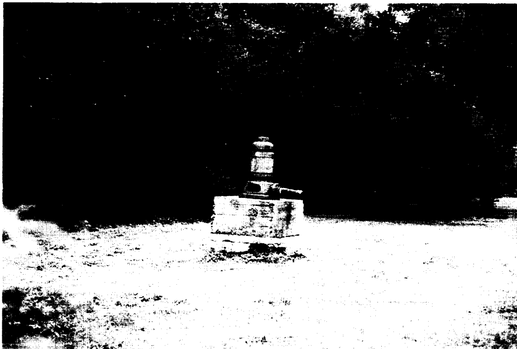
FIGURE 3-6. Land subsidence away from the wellhead located near the Burnett School in Baytown, Texas.
