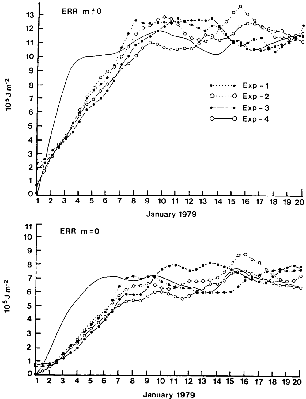
Figure 4 Growth of prediction errors in the four simulations: ERR_{m \neq 0} is eddy baroclinic ( n = 1-15 , m = 1-10 ) components, and ERR_{m = 0} eddy barotropic ( n = 1-15 , m = 0 ) components. The simulations are distinguished by coarse (dashed line) and fine (solid line) model resolutions with a combination of GLA (black dot) and GFDL (white dot) initial datasets. Persistence errors starting from 1 January 1979 are presented by a solid line without symbols.
