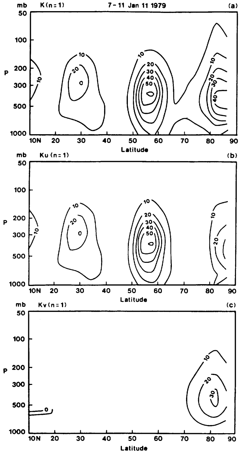
FIG. 9. Meridional-height cross sections of kinetic energy K , zonal component K_w and meridional component K_v in the Northern Hemisphere for n = 1 . The values are 5-day means for 7-11 January 1979, multiplied by \rho_0 and expressed in the units of J m^{-3} .
