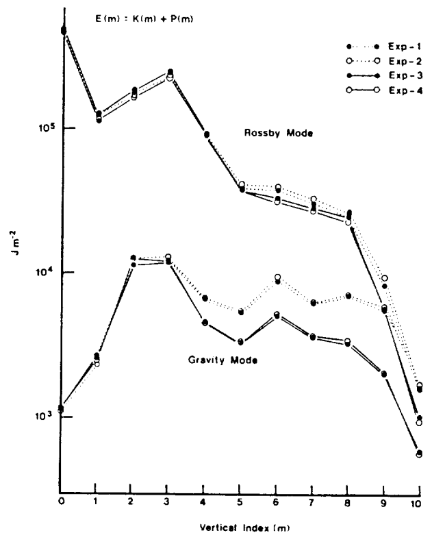
Figure 3 As in Figure 2, but in the vertical index domain m = 0-10 .
