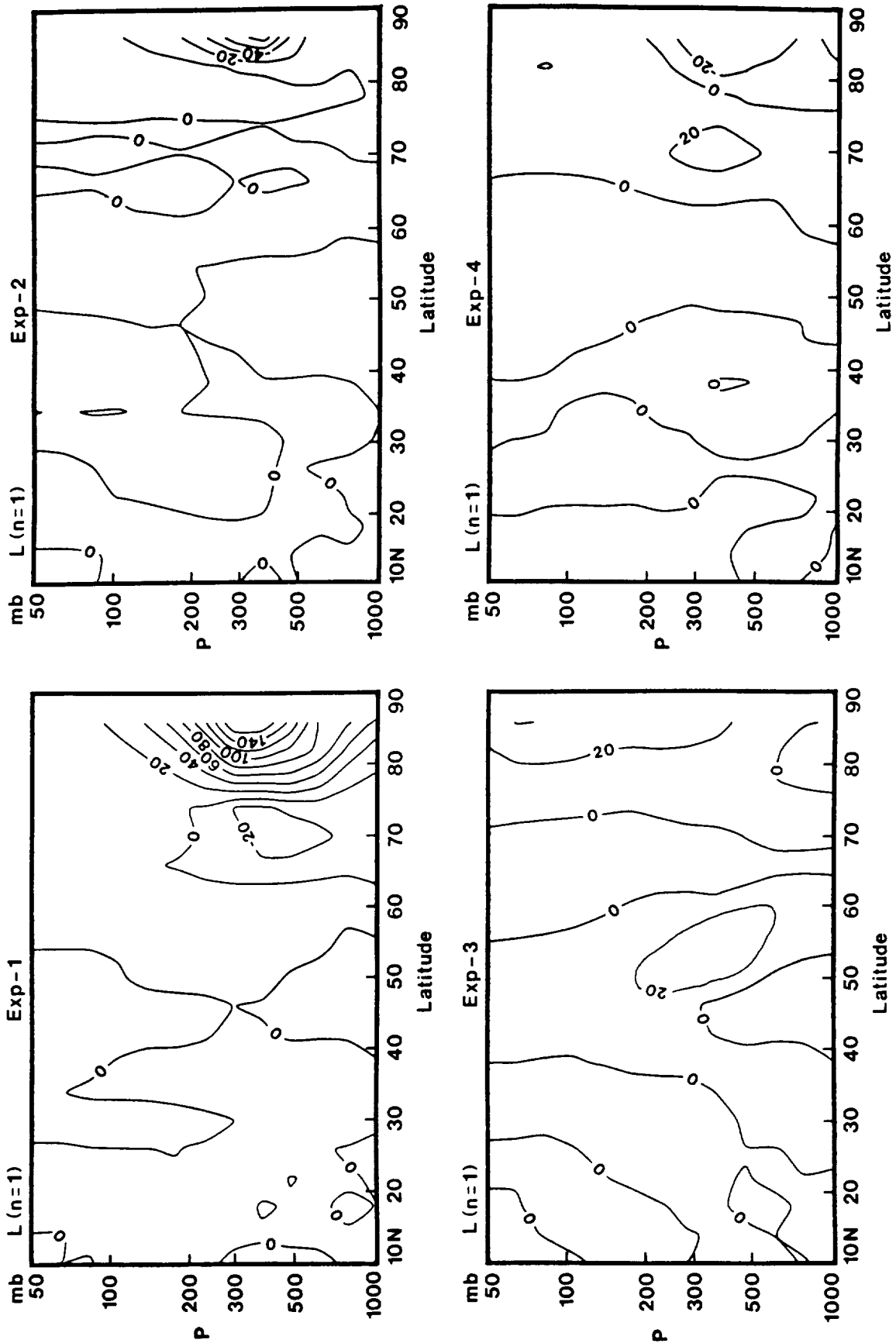
FIG. 13. As in Fig. 12, but for the wave-wave interaction.
