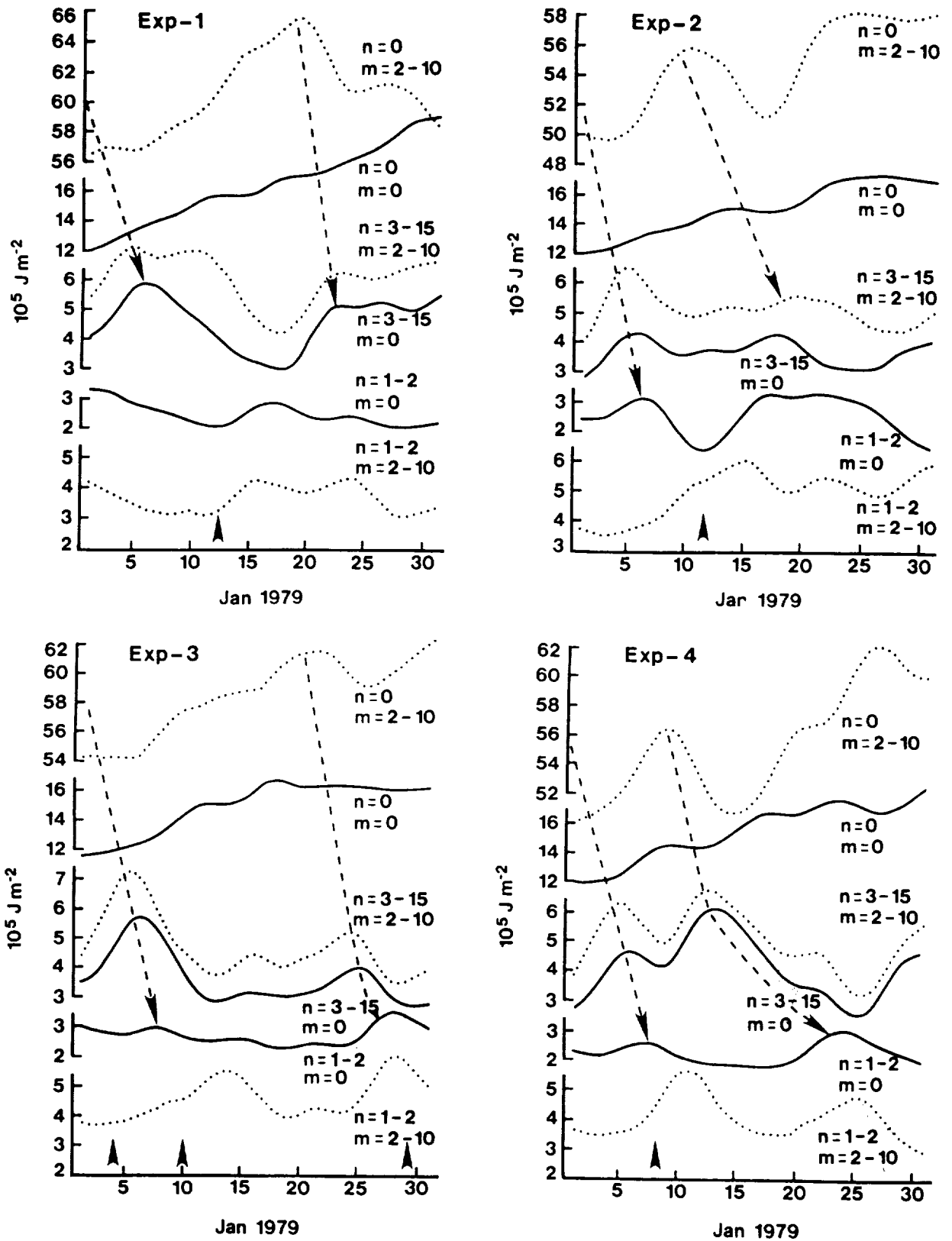
FIG. 15. As in Fig. 14, but for the four simulations. Baroclinic energy is the sum of baroclinic indices m = 2-10 .
