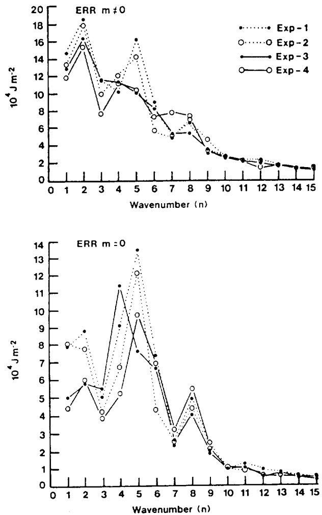
Figure 5 Error energy spectra of the four simulations on date 7: \text{ERR}_{m \neq 0} is baroclinic ( m = 1-10 ) components, and \text{ERR}_{m = 0} barotropic ( m = 0 ) components.
