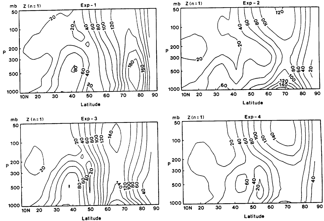
Figure 8 As in Figure 7, but for the four simulations during the same period.
