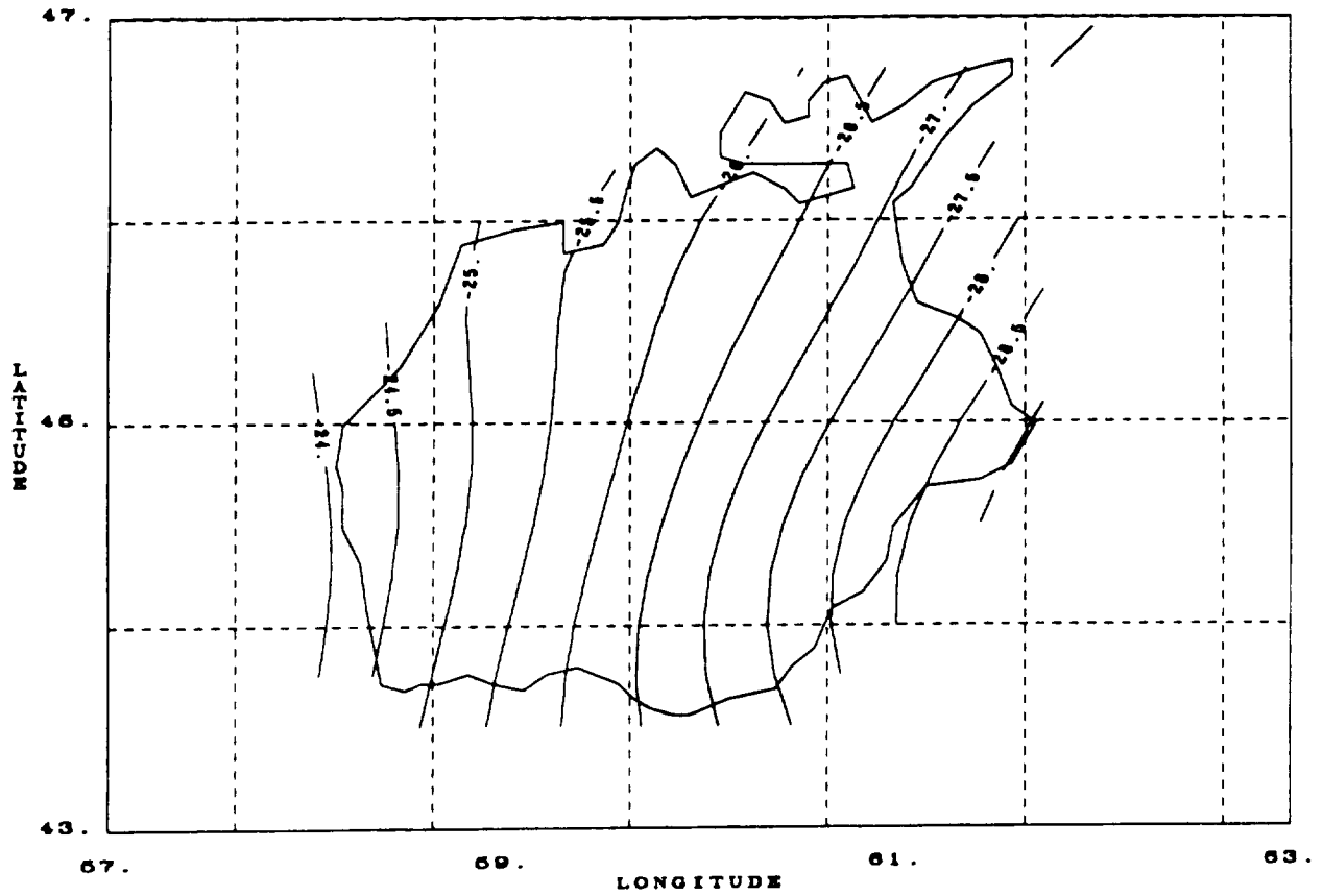
Figure 5. A contour map of Rapp's 180 x 180 reference geoid undulations (m above mean sea level) of the Aral Sea.
