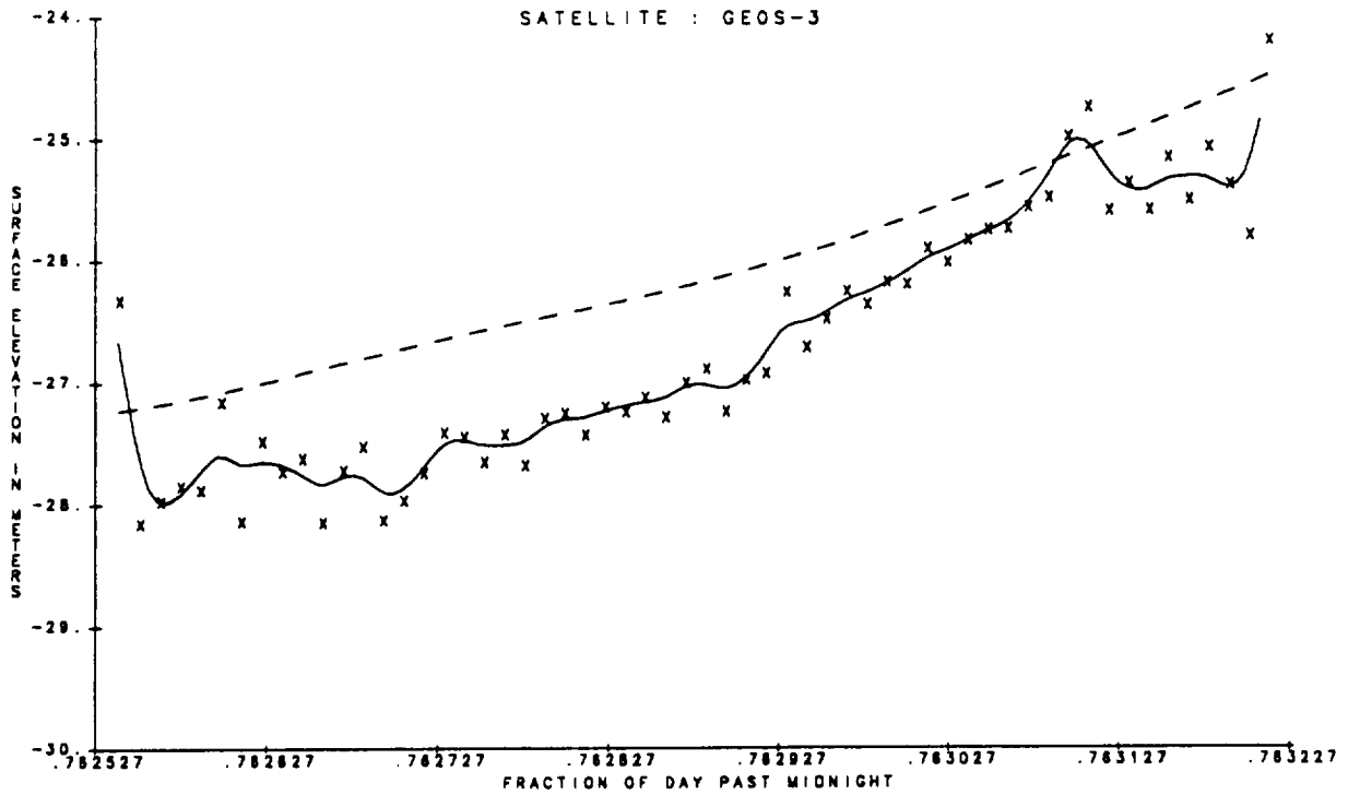
Figure 3. Sample adjusted altimeter elevation profile of the Aral Sea--profile of the reference pass. Dashed line is the Rapp's 180 x 180 reference geoid.
