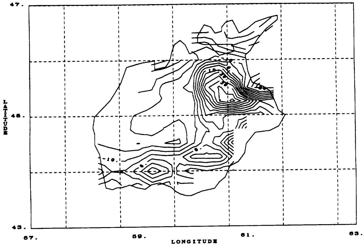
Figure 12. A contour map of estimated gravity anomalies of the Aral Sea predicted with local empirical covariance functions.
