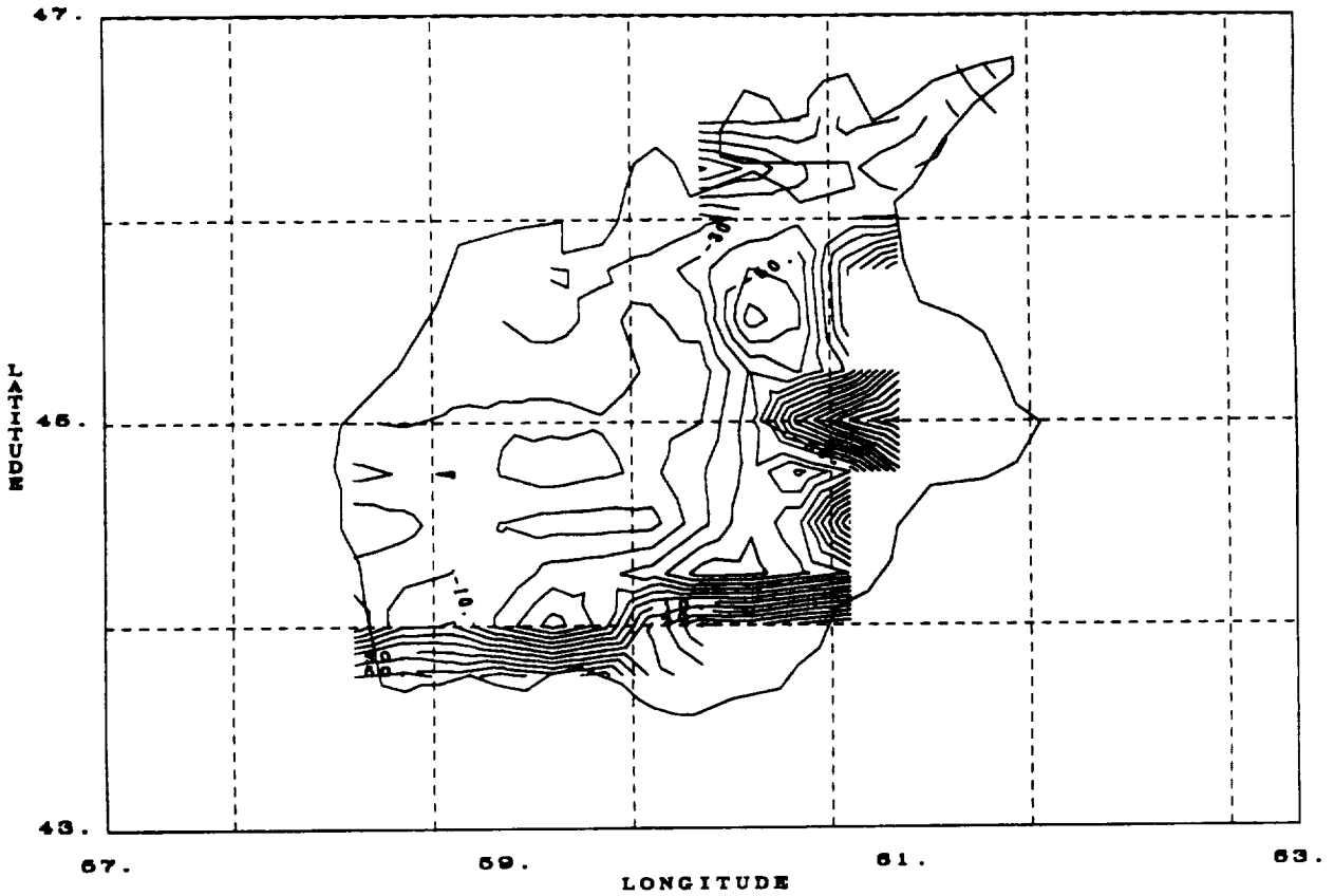
Figure 14. A contour map of estimated gravity anomalies of the Aral Sea predicted with Jordan's covariance functions.
