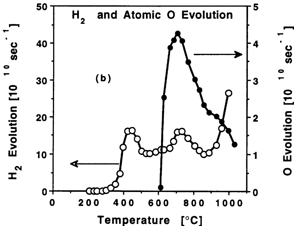
Fig. 6a/b Evolution of H 2 O, H 2 and O during decomposition in vacuum of ultrahigh purity Mg(OH) 2 into MgO. Note that the intensity scales for H 2 O, H 2 and O differ as 1000:10:1 (after [Martens et al., 1976]).
