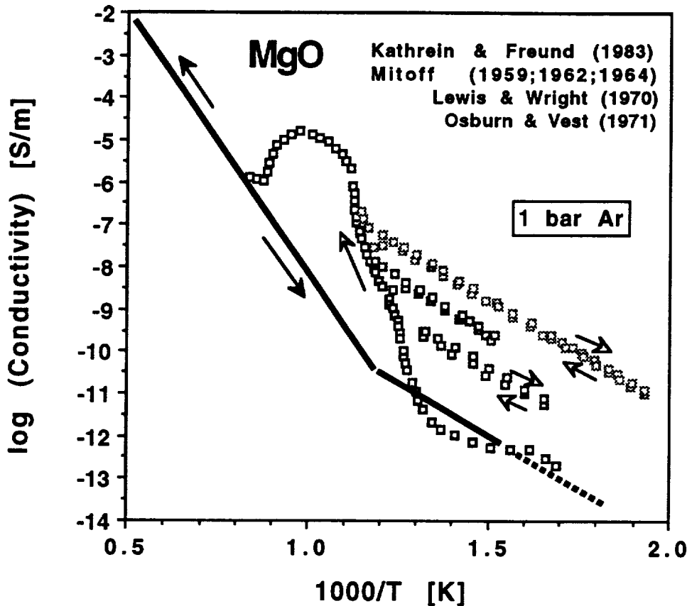
Fig. 2 Typical electrical conductivity behavior of high purity, arc-fusion grown MgO single crystals heated in high purity Ar. The data represented by open squares are adopted from Kathrein and Freund (1983) . The small maximum below 400°C ( 1000/T > 1.5 ) was confirmed by Kathrein et al. (1980) . The steep section of the solid line delineates the high temperature Arrhenius branch as reported by many authors including Mitoff (1959, 1962, 1964) , Lewis and Wright (1970) and Osburn and Vest (1971) . The less steep section and dashed extension is adopted from graphical representations given by Lewis and Wright (1970) and from work by Kathrein and Freund (1983) .
