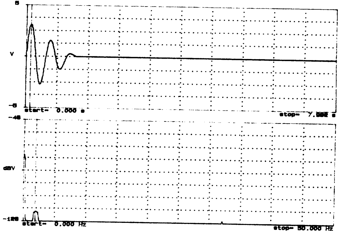
Figure 9. Bare Cuff (concluded)
