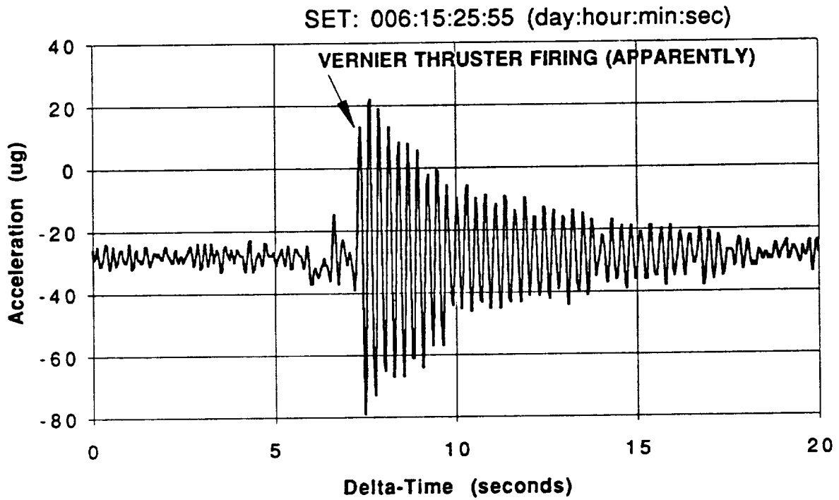
(c) Acceleration versus time (TSH-A, y-axis).
