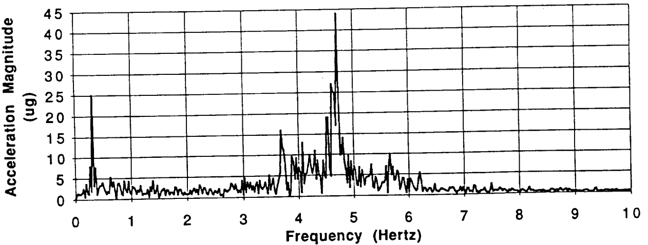
(a) Acceleration versus frequency.
