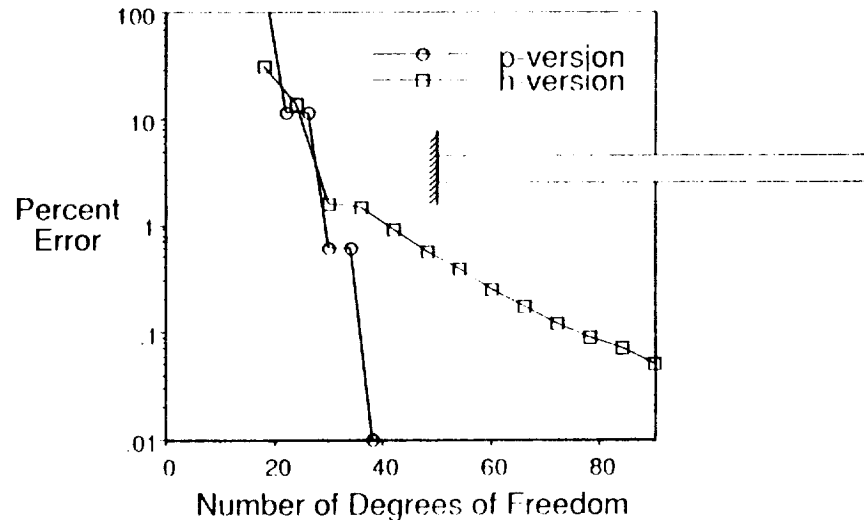
Percent Error vs Number of Degrees of Freedom. Fifth bending frequency
