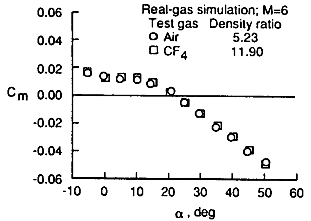
Figure 9. Hypersonic aerodynamic real-gas effects.
