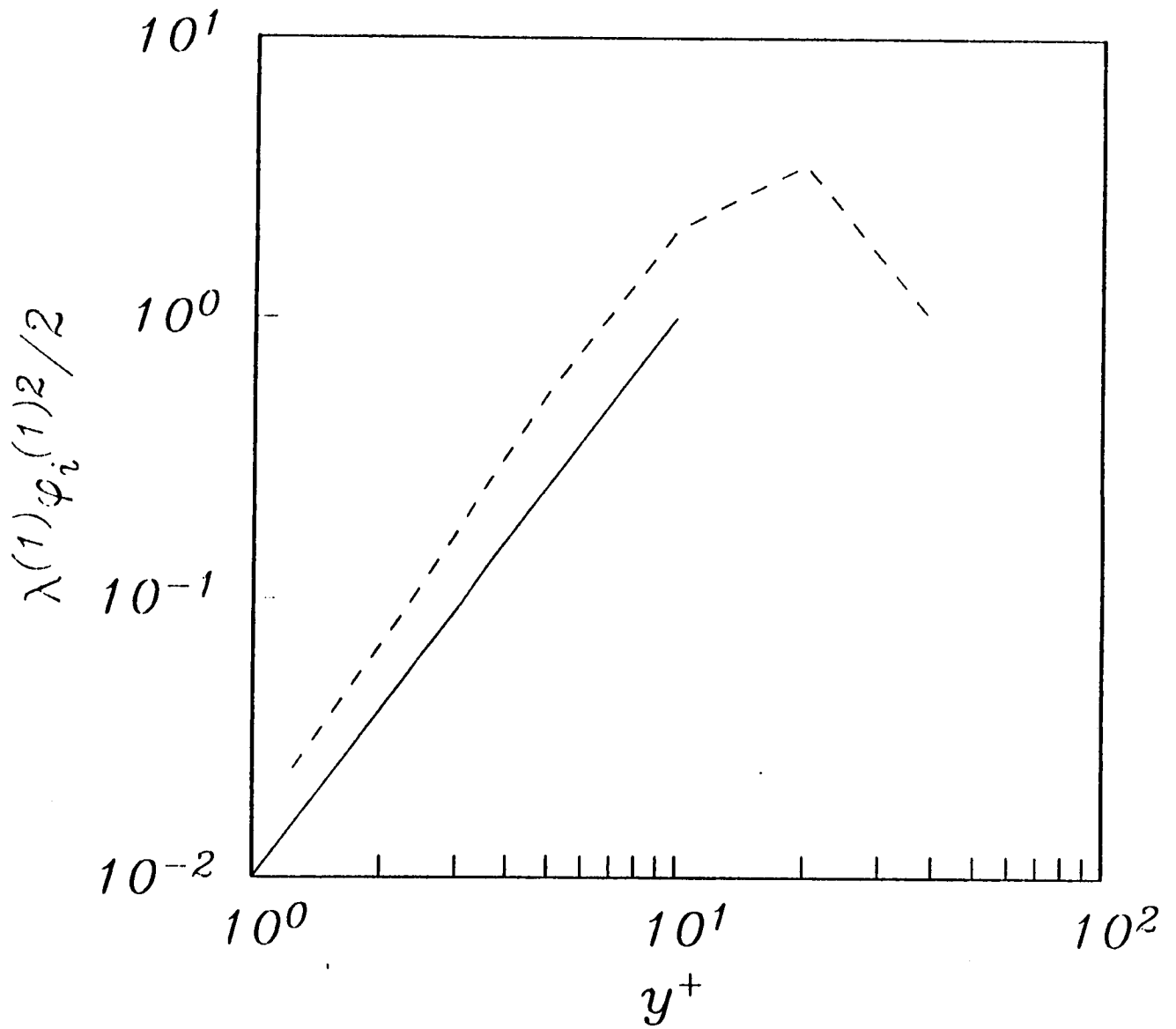
Figure 1. One mode contribution to the turbulent kinetic energy.
