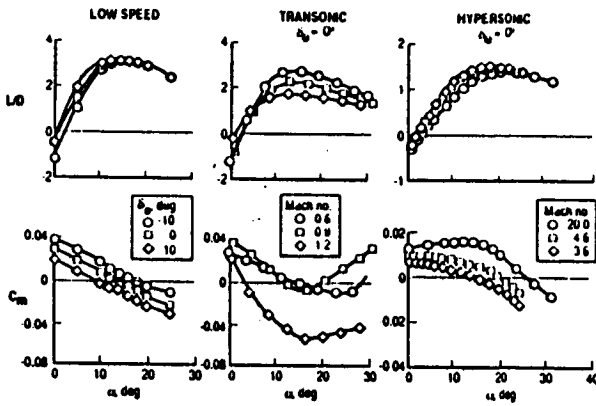
Figure 8. PLS longitudinal aerodynamic characteristics (moment ref. = 0.54L).
