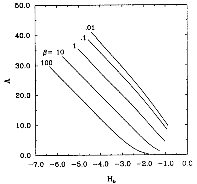
Figure 4.—The amplitude A of the stable localized state as a function of the logarithm of the background thickness, \log_{10}(H_b) , for various values of \beta . Note that these curves are nearly linear.
