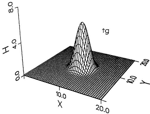
(a) A = 5.7874 , H_b = 6.2789 \times 10^{-2} , \lambda = 1.9507 .
