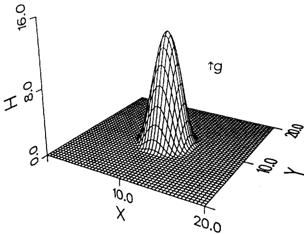
(b) A = 13.6065 , H_b = 6.5057 \times 10^{-3} , \lambda = 4.0542 .
