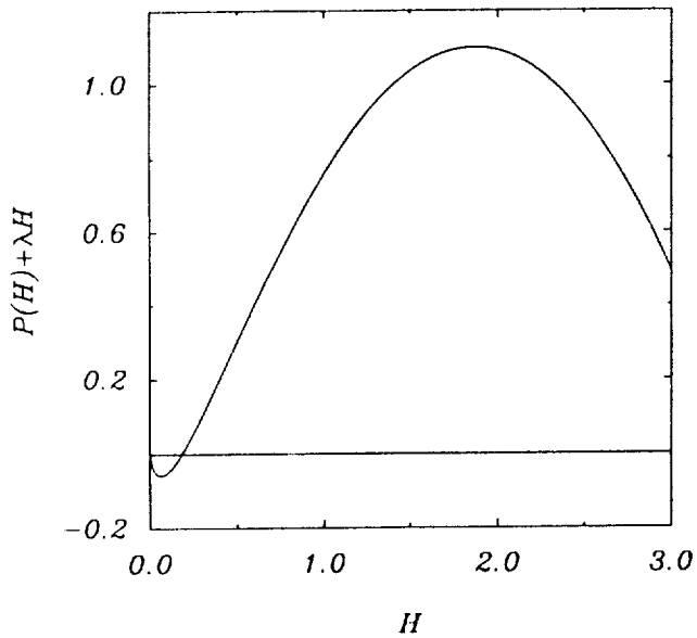
Figure 3.—The effective potential P(H) + \lambda H for the localized state shown in Fig. 1a, as a function of H . The value of \lambda = 1.90507 is calculated using eq. (8). The background thickness H_b = 6.2789 \times 10^{-2} lies in the minimum of the potential well.
