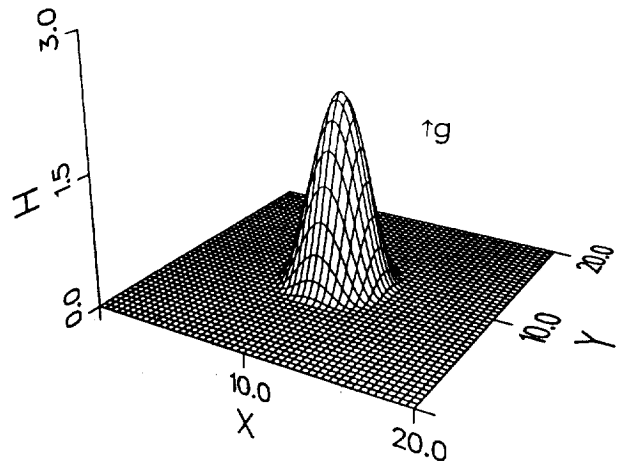
(b) \beta = 100 .
