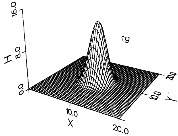
(a) \beta = 0.01 .
