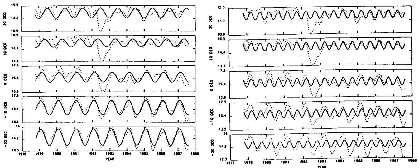
Fig. 1. Mid-stratospheric 10mb Ozone Mixing Ratio Variations (μmb/mb) at equatorial and subtropical latitudes (Oct 79 – Sep 87)
