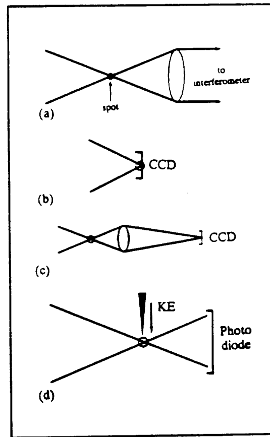
Figure 1. Measurement methods: (a) interferometric; (b) CCD direct; (c) CCD with aux. lens; (d) knife-edge scanner.
