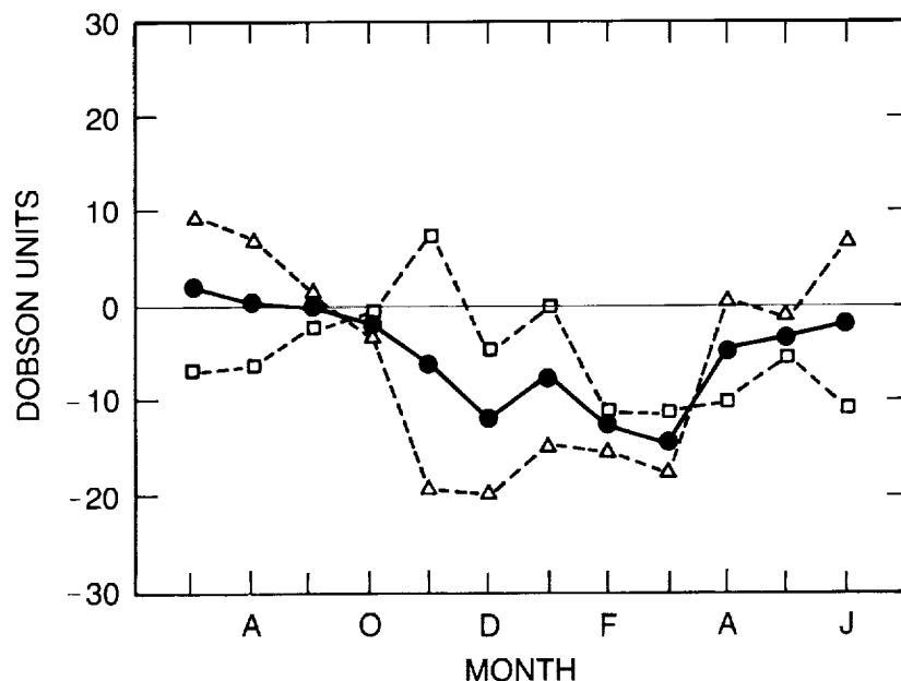
Figure 4.54 The points using the symbol ● are the differences in the monthly averages for the periods January 1963–December 1974 and January 1975–December 1986 for a combined series of the data from Belsk and Bismarck. The equivalent results when only Belsk was taken as operating in the former period are shown with the symbol □, while those for the case where just Bismarck was taken for the first period have the symbol ▲. In all cases, both stations' data were used in the second period.
