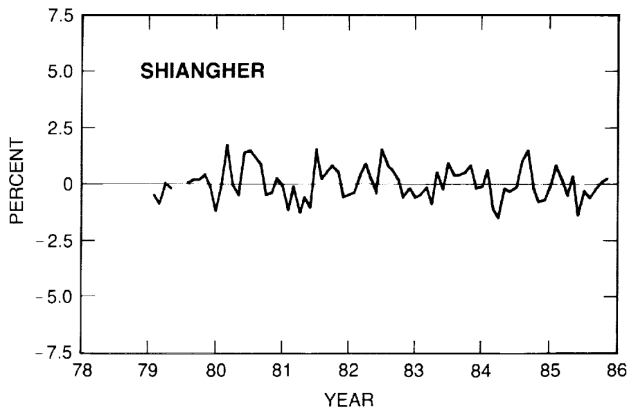
Figure 4.13 Monthly (Dobson-TOMS)/Dobson differences for Shiangher (near Beijing). The \sigma of the differences forming each monthly point is about 2.1 percent. The circles and the solid curves indicate direct-Sun observations.
