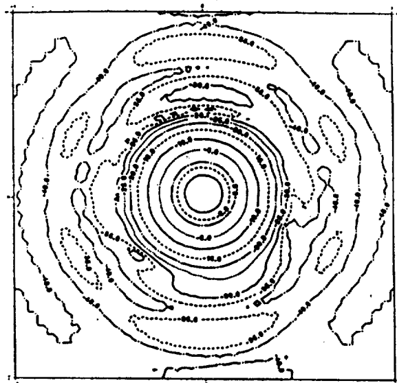
Figure 4a, Ideal Case Far-Field Antenna Pattern
