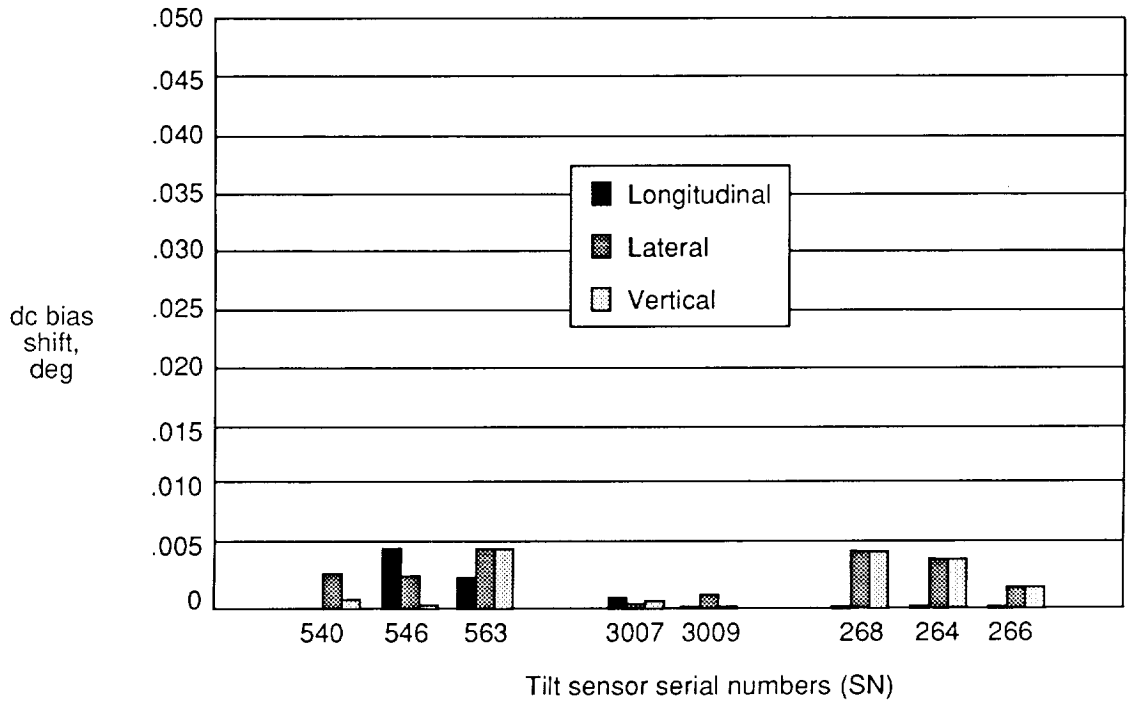
Figure 40. Random rectification test showing dc bias shift of tilt sensors at 2g rms at level position.
