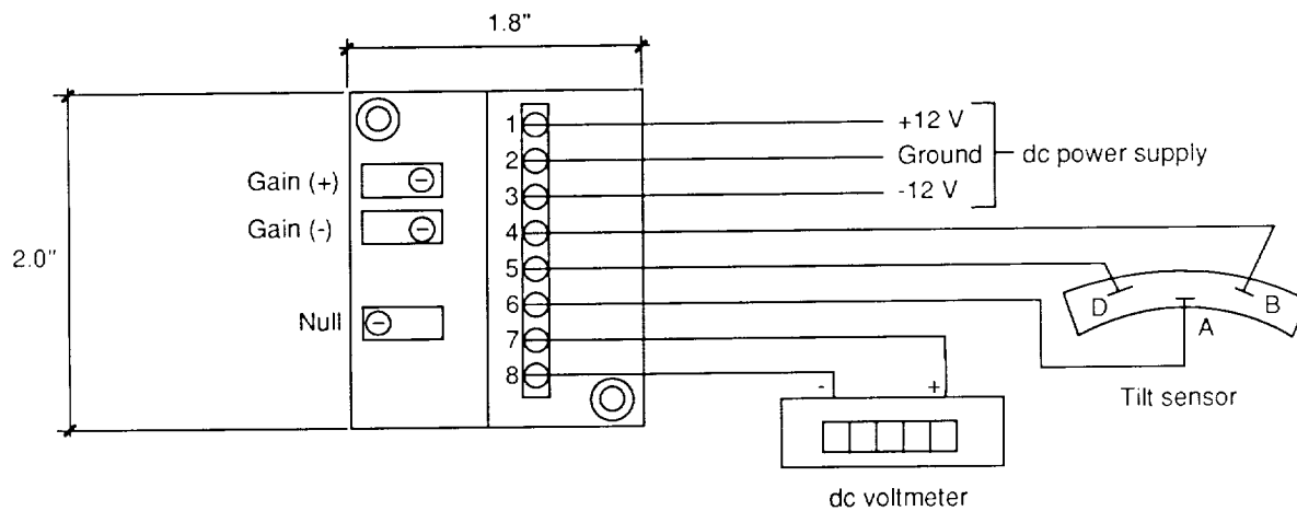
Figure 3. Signal conditioning module.
