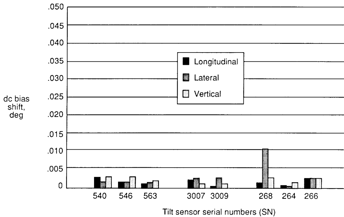
Figure 45. Random rectification test showing dc bias shift of tilt sensors at 1g rms at -5° tilt level.
