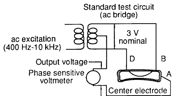
(c) Electrical schematic drawing.
