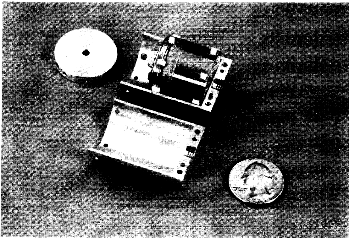
(b) Disassembled servo accelerometer package.
