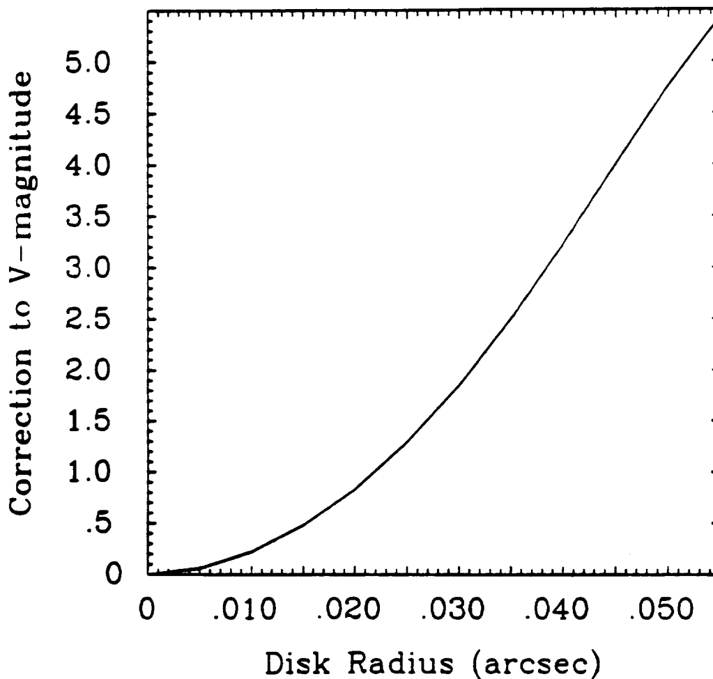
No Limb Darkening
