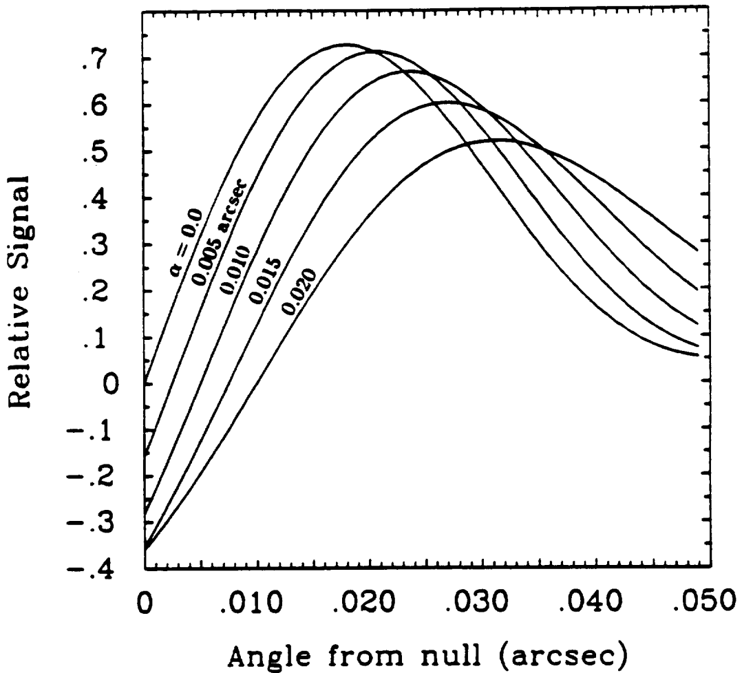
Transfer Function for close binaries
