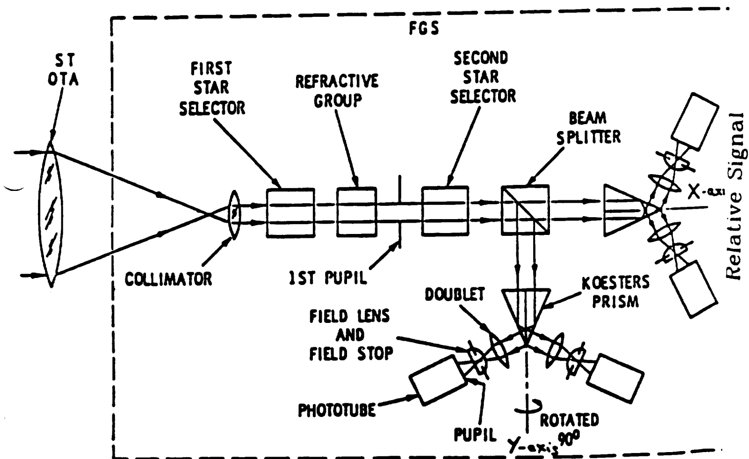
SIMPLIFIED FGS OPTICAL SCHEMATIC
