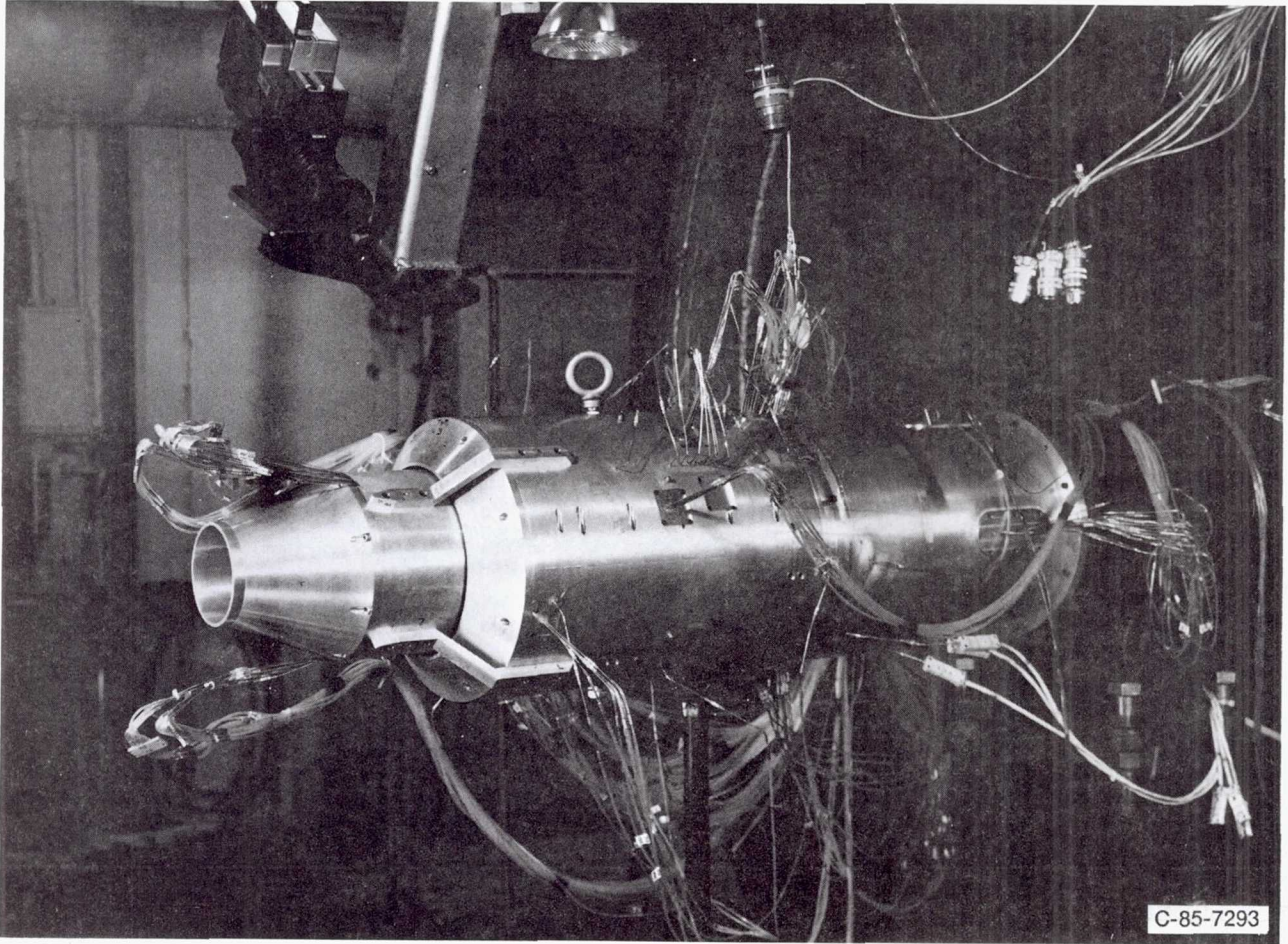
Figure 1.—Typical model installation.
