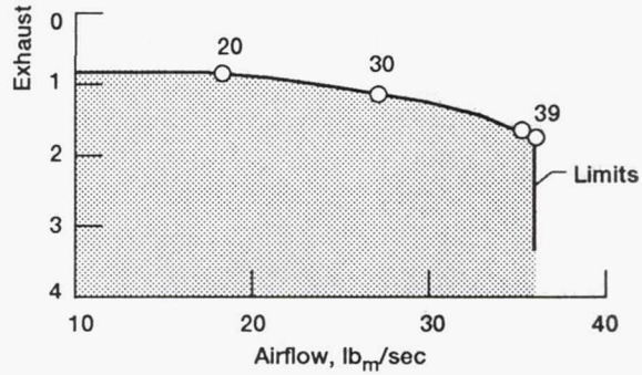
(b) 40-in. 2 throat ASME nozzle.
