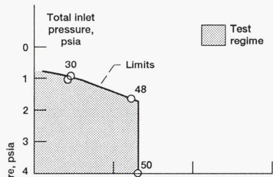
(a) 20-in. 2 throat ASME nozzle.
