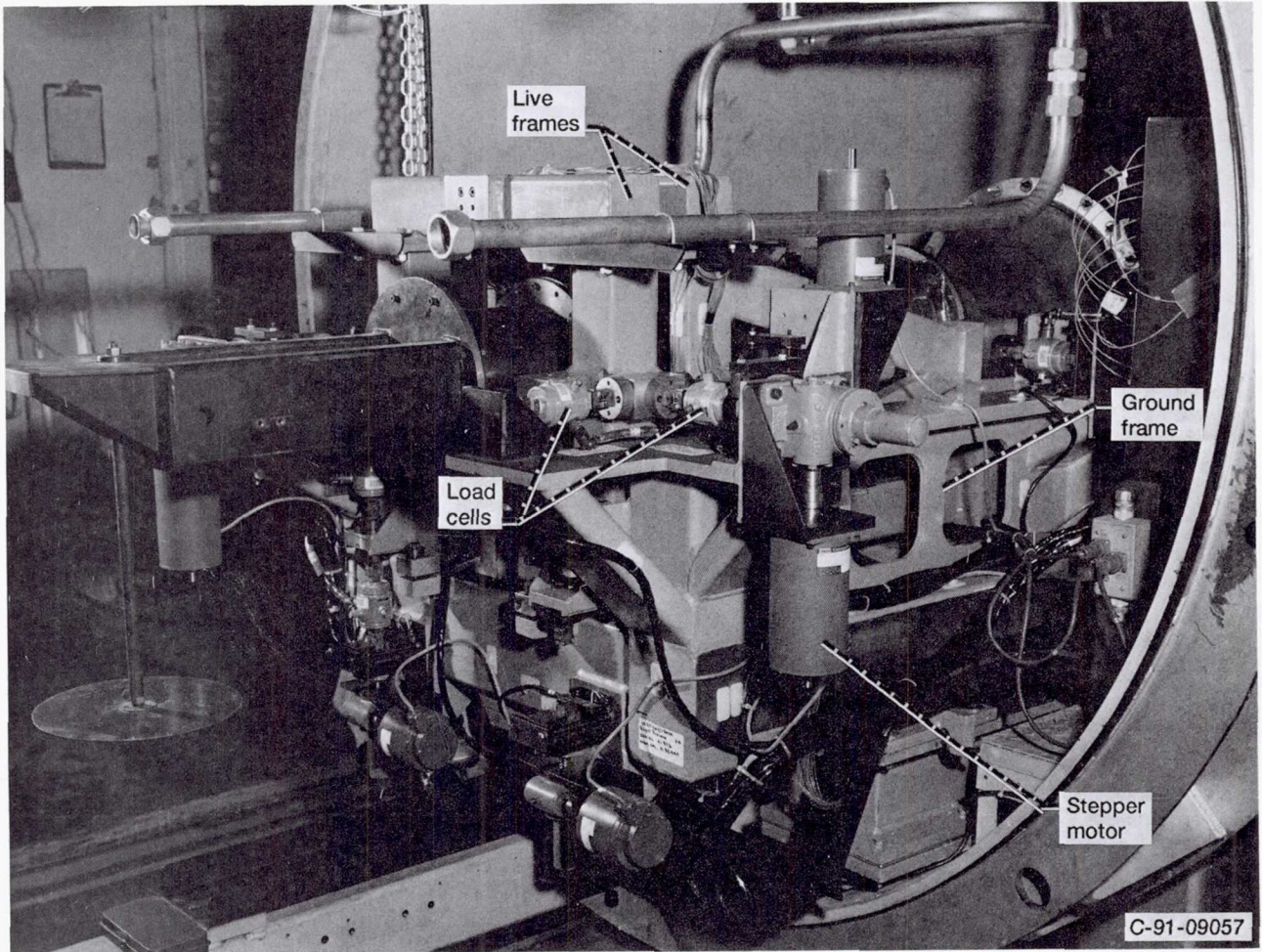
Figure 7.—Thrust and flow measurement systems.
