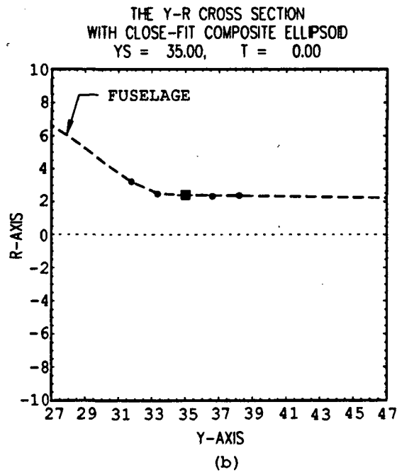
Figure 4.14: A close-fit composite ellipse in the YR-plane for the antenna located at (Y_s, T) = (35, 0) .
