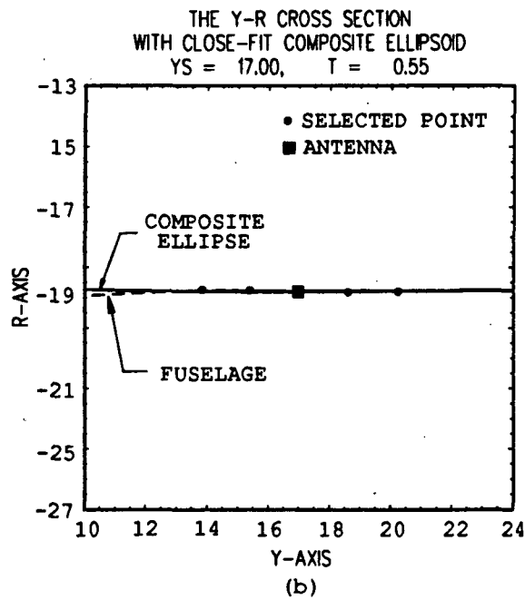
Figure 4.2: A close-fit composite ellipse in the YR-plane for the antenna located at (Y_s, T) = (17, 0.55) .
