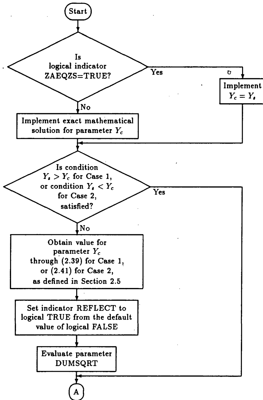
Figure 3.11: A simplified flow-chart for subroutine SRRO.
