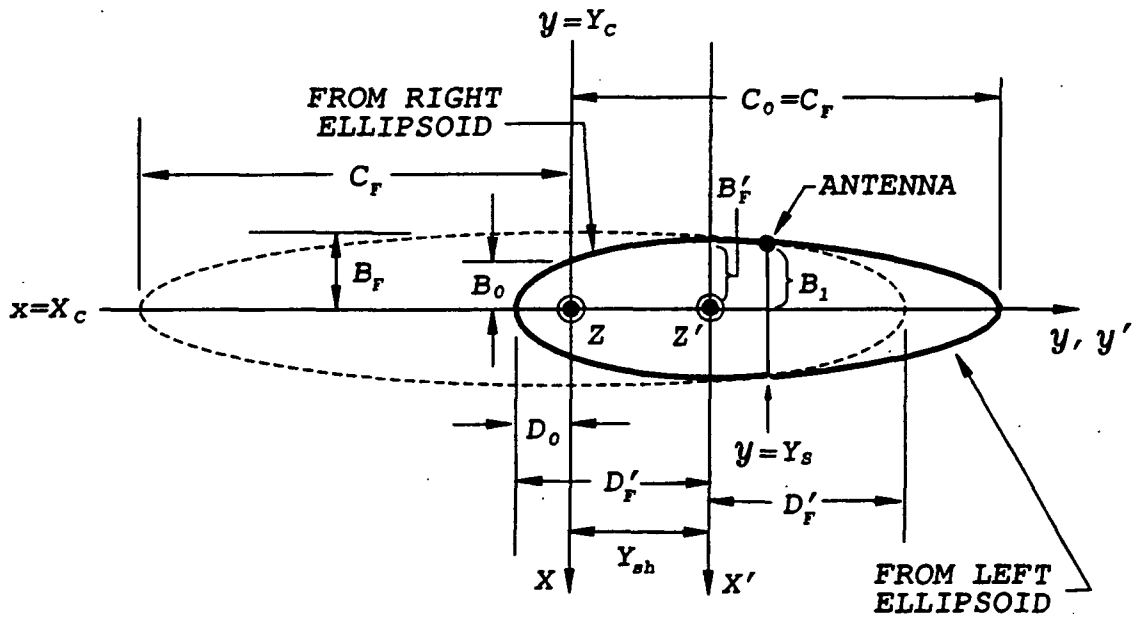
(b) CASE 1 ( Y_s \geq Y_c ): TOP VIEW
