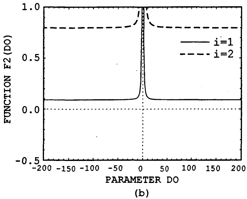
Figure 4.15: Plots of function f_{2_i} (for i = 1, 2 ) for the antenna located at (Y_s, T) = (35, 0) prior to perturbation in the YR-plane.
