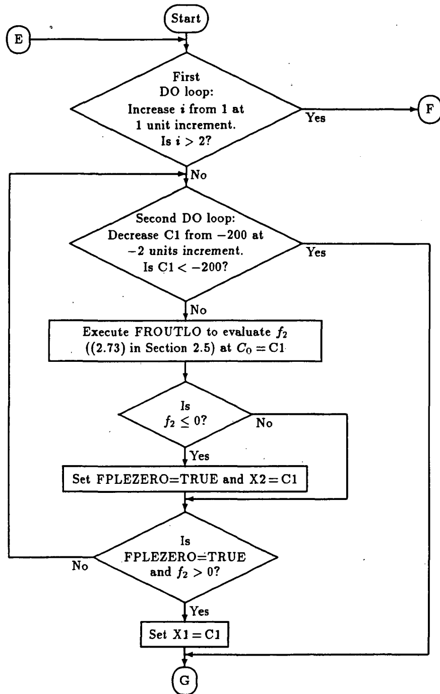
Figure 3.18: A simplified flow-chart for subroutine RTSAFE0.
