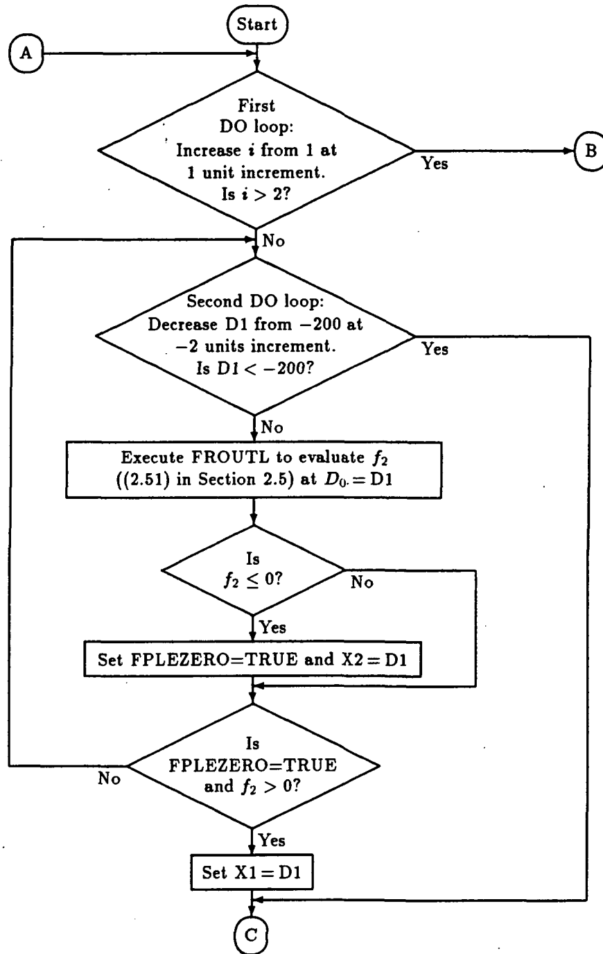
Figure 3.15: A simplified flow-chart for subroutine RTSAFE.
